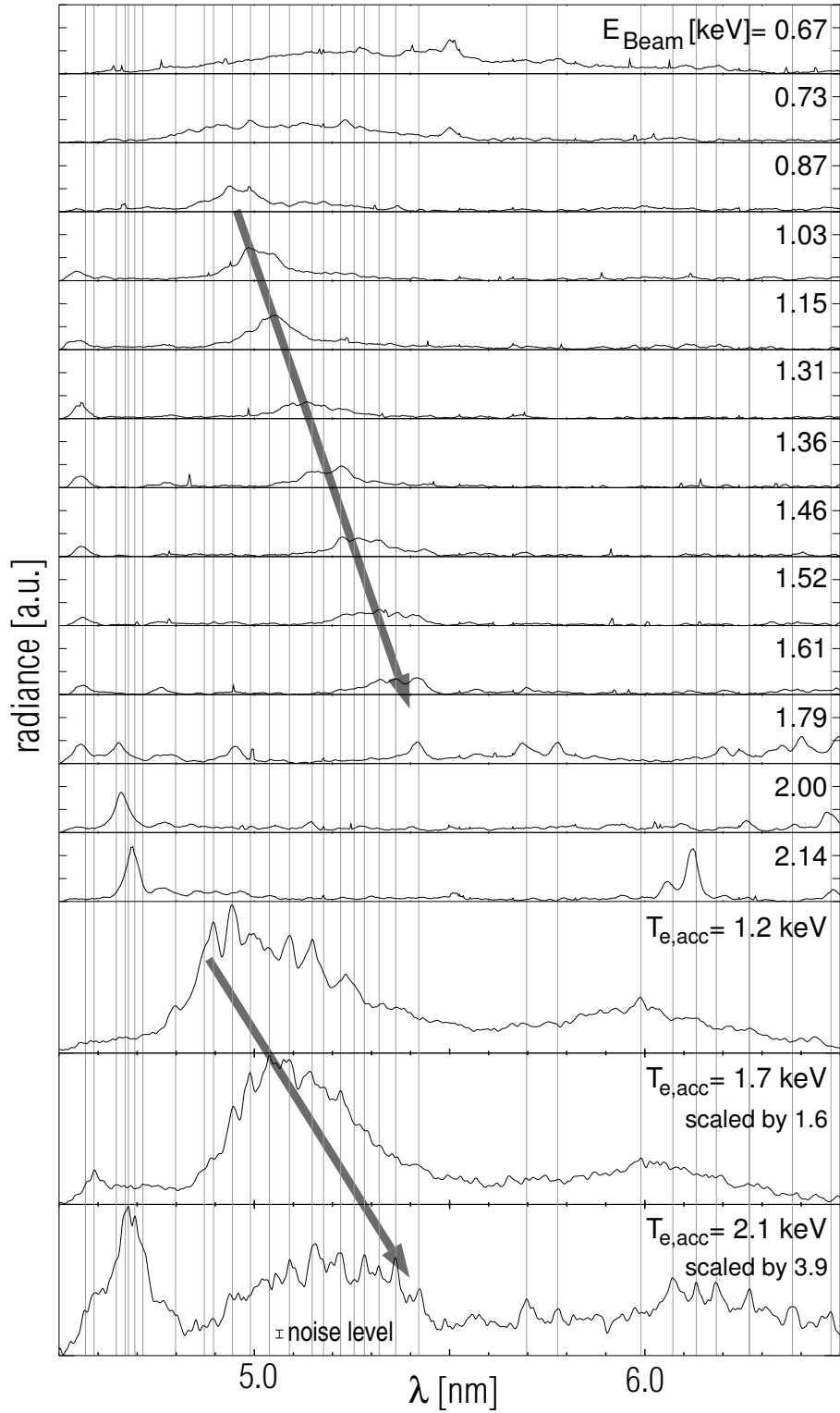
Figure 6.2: EBIT spectra for several electron beam energies compared with tokamak spectra from ASDEX Upgrade discharge #19436 with impurity accumulation. Vertical lines are drawn to guide the eye. For better display, the tokamak spectra for T_{e,\text{acc}}=2.1 keV ( t=6.53 s) and T_{e,\text{acc}}=1.7 keV ( t=6.60 s) are scaled relatively to the spectrum for T_{e,\text{acc}}=1.2 keV ( t=7.00 s) by factors 3.9 and 1.6, respectively. EBIT spectra are not scaled relative to each other to give an impression of the relative strength of emissions which are superimposed in the tokamak spectra.
