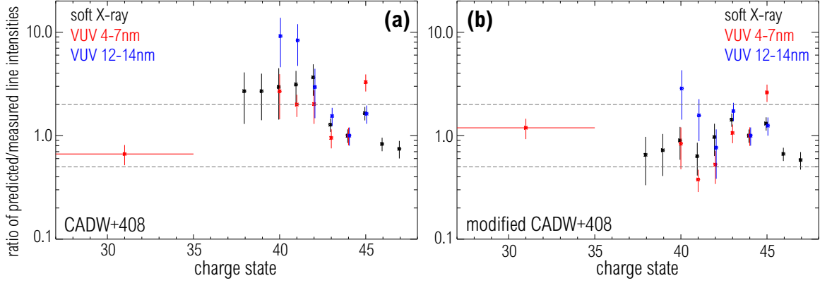
Figure 5.8: (a) Ratios of predicted over measured line intensities for different wavelength ranges versus ionization state using the 'CADW+408' ion balance (s. figure 5.3, 5.4, 5.5 and 5.9). All lines of an ionization state are summed in the model and in the spectrum to mitigate the uncertainties that would occur for a single spectral line. (b) Similar data to part (a) of the figure, but using modified 'CADW+408' data. The modifications are described in the text.
