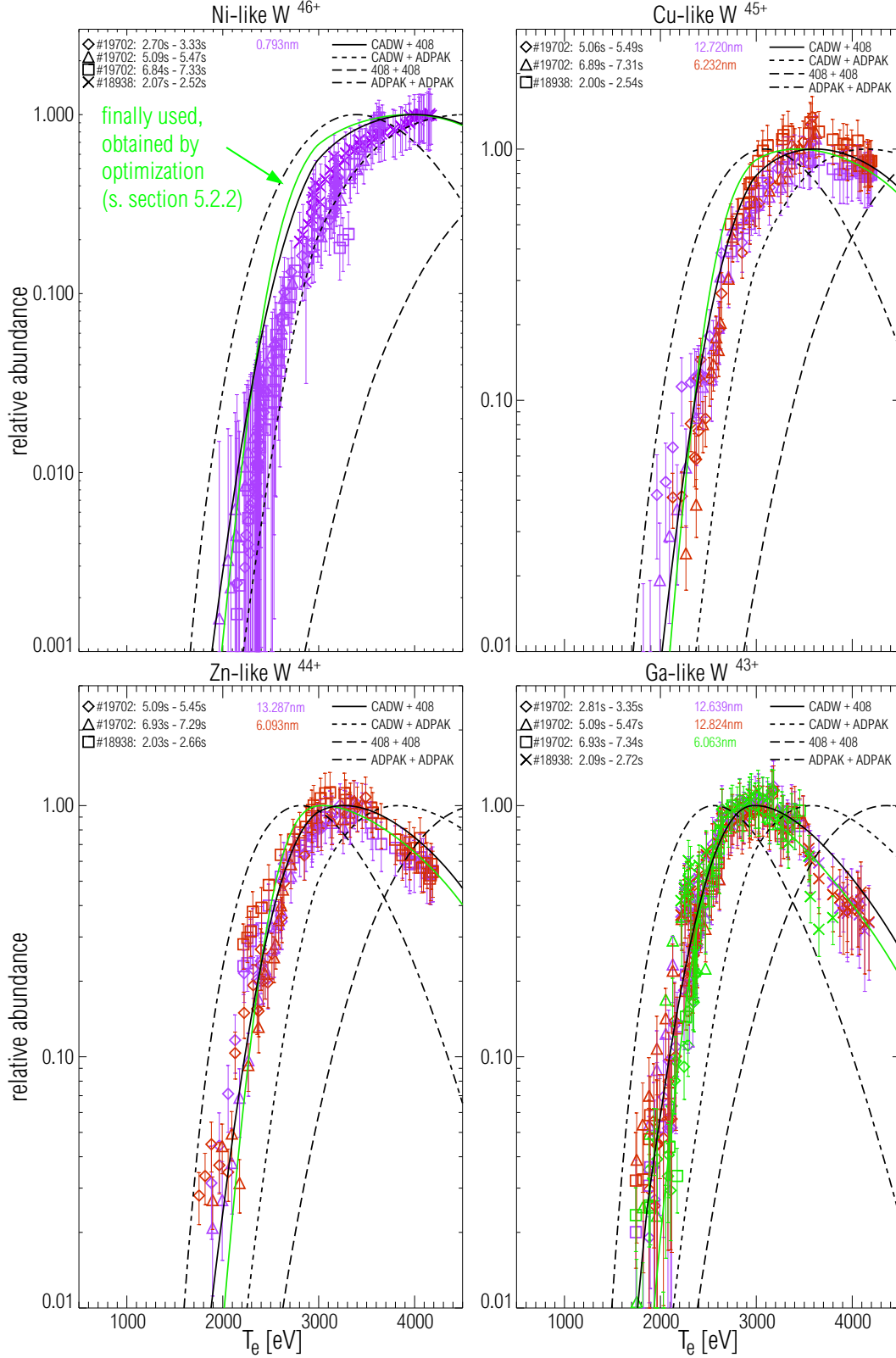
Figure 5.3: The relative abundances of Ni-like W ^{46+} to Ga-like W ^{43+} derived from theoretical data (lines) and from measurement (symbols). Measurements originate from impurity accumulation phases. The data are color coded indicating the analyzed spectral lines. The uncertainty in electron temperature is \pm 200 eV. The legend is featuring the underlying ionization and recombination data by abbreviations on the left and on the right of the '+', respectively. 'CADW' = configuration average distorted wave data (s. section 2.3.3), '408' = ADAS baseline data using level-resolved calculations from the Cowan code, 'ADPAK' = data from the average ion model [25], which were modified in [39] according to experimental findings. The green line is the result of a modification of the 'CADW + 408' data, which will be explained in section 5.2.2
