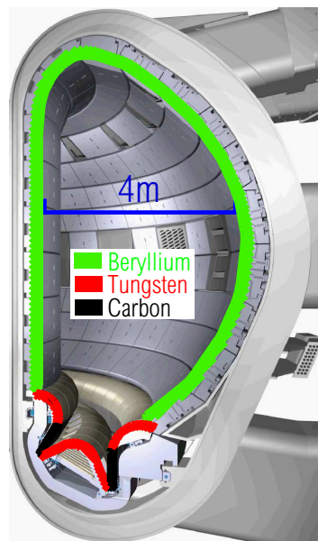
Figure B.3: ITER cross section showing actual plans for plasma facing components
