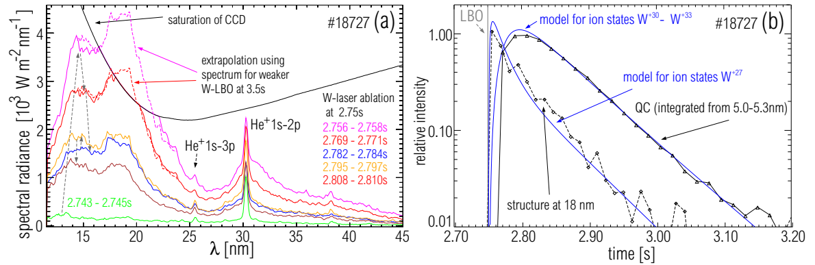
Figure 6.11: (a) Spectra before and after a laser ablation of tungsten featuring a broad structure around 18 nm. The first two spectra have been extrapolated using spectra of laser ablations involving less tungsten, due to a partial saturation of the measurements. (b) Measured evolution of the emissivities after a laser ablation. The presented traces (black using additionally symbols) correspond to the signal integrated in the interval 16–22 nm (structure at 18 nm) and the interval 5.0–5.3 nm (central part of the quasicontinuum). The blue traces denote the integral of the charge state densities along the LOS for the stated charge states for the modeled plasma. Modeled behavior was obtained by STRAHL.
