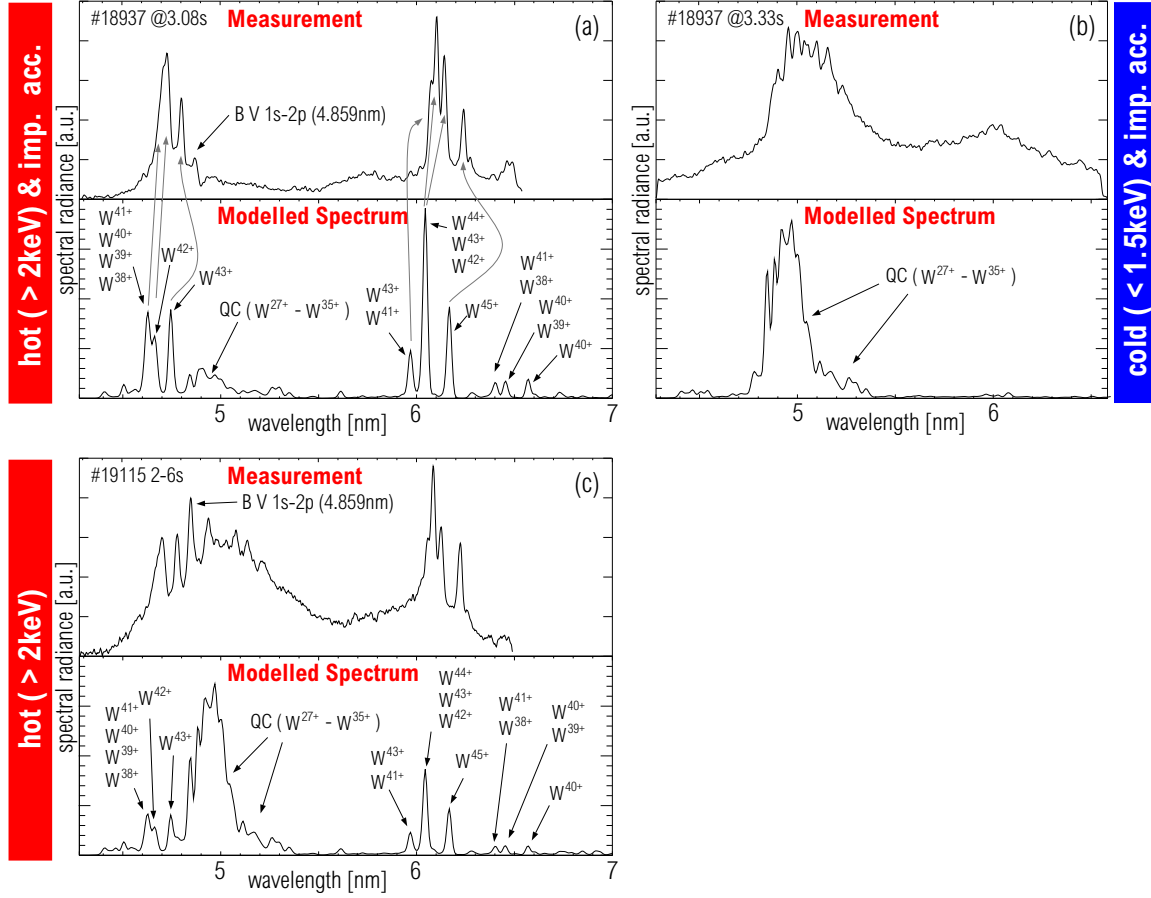
Figure 6.5: (a) Measured and modeled spectra for an impurity accumulation phase, in which the accumulation region exhibited a temperature of \approx 3 \text{ keV} . The radiation profile is peaked in the center by a factor of about 25, therefore, the quasicontinuum (QC) is strongly suppressed in comparison to the other emissions in the spectrum. The spectral lines start to emerge in the spectrum for temperatures above 2 keV. The modeled spectra were obtained using ADAS data. (b) as (a) but for electron temperatures below 1.5 keV (c) Measured and modeled spectra for discharge #19115 with an approximately flat tungsten concentration and a central electron temperature of \approx 3.6 \text{ keV} .
