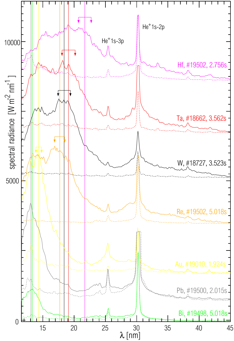
Figure 7.3: Spectral signatures of _{72}\text{Hf} , _{73}\text{Ta} , _{74}\text{W} , _{75}\text{Re} , _{79}\text{Au} , _{82}\text{Pb} and _{83}\text{Bi} following a LBO. An arbitrary offset is added to the spectra of each element for better display. Dashed spectra correspond to a timepoint directly before the LBO. The different absolute size of the emissions are caused by the different amount of the injected impurity, which might vary for each element due to the efficiency of the impurity injection by laser ablation.
