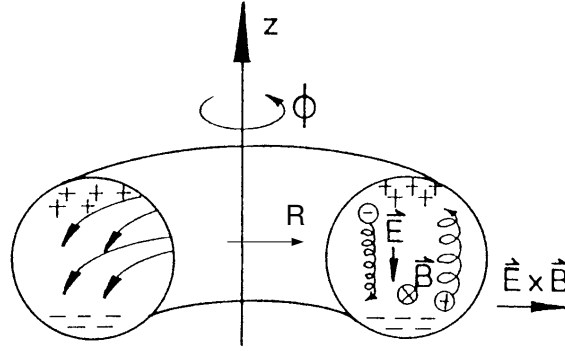
Figure A.1: Sketch of charge distributions and E \times B drift for a purely toroidal magnetic field
