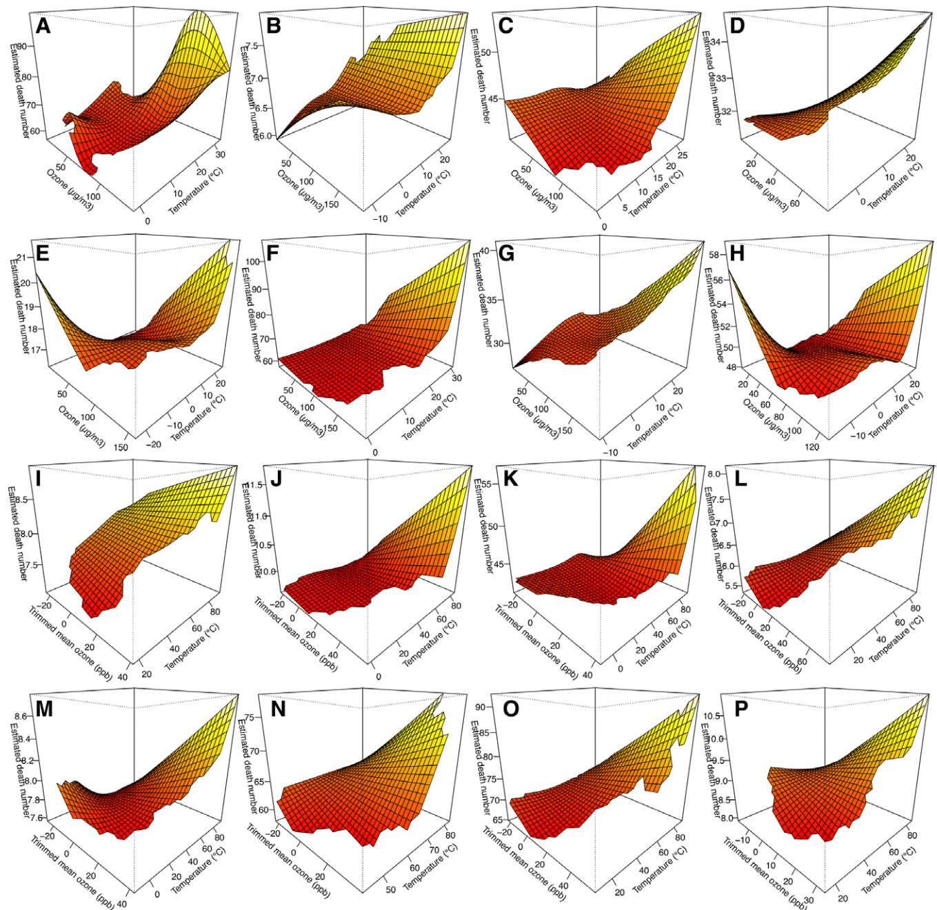
Figure 1. Bivariate response surfaces for ozone and temperature on daily mortality. A, Athens, Greece; B, Augsburg, Germany; C, Barcelona, Spain; D, Copenhagen, Denmark; E, Helsinki, Finland; F, Rome, Italy; G, Ruhr, Germany; H, Stockholm, Sweden in Europe; I, Atlanta, GA; J, Buffalo, NY; K, Chicago, IL; L, DC; M, Kansas city, MO; N, Los Angeles, CA; O, New York, NY; and P, Seattle, WA, in the United States.
