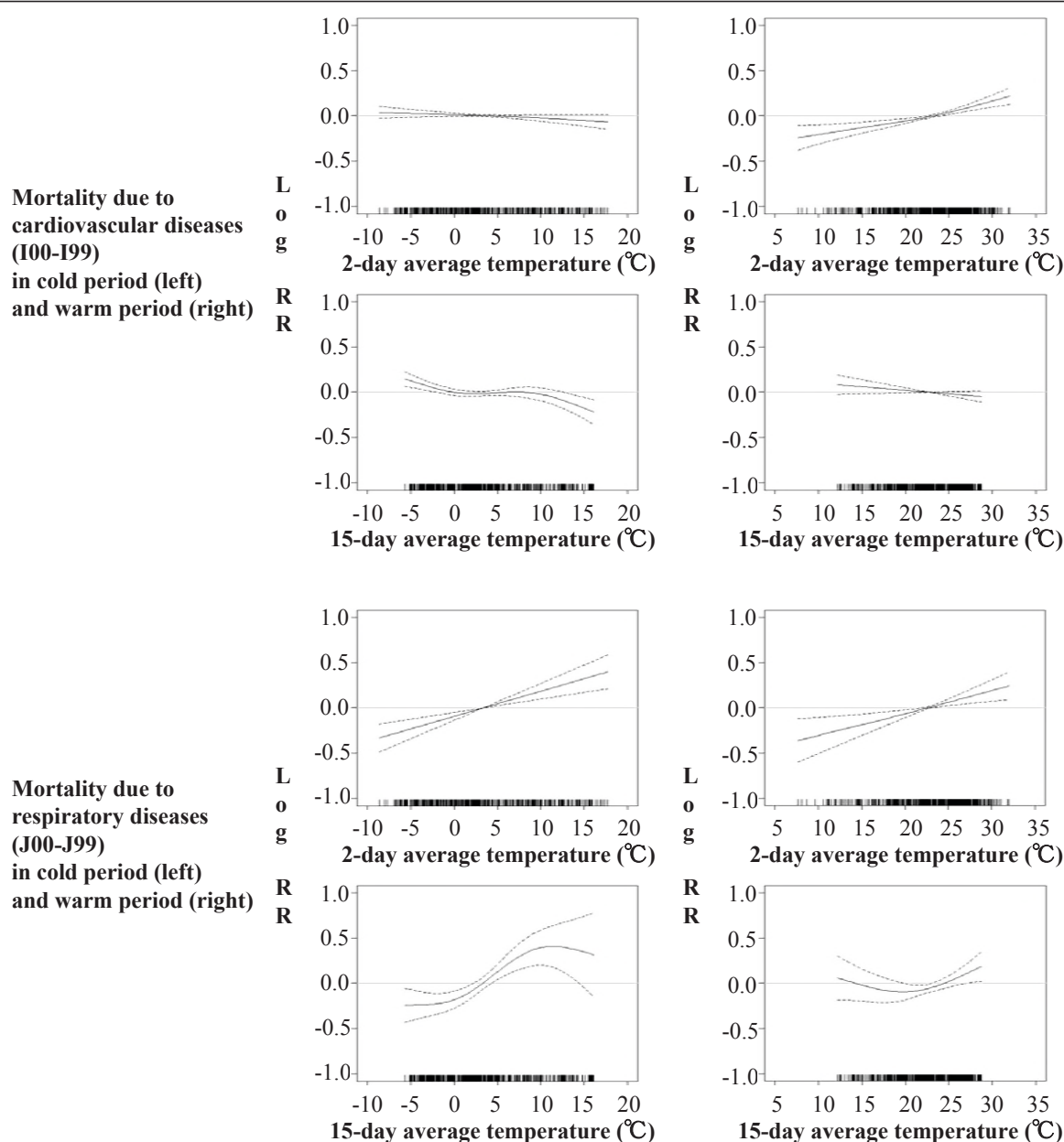
Figure 2 Exposure-response functions (together with 95% CIs) for two-day and 15-day average temperature and daily mortality of the whole population due to cardiovascular and respiratory diseases in the urban area of Beijing, by warm/cold period.
