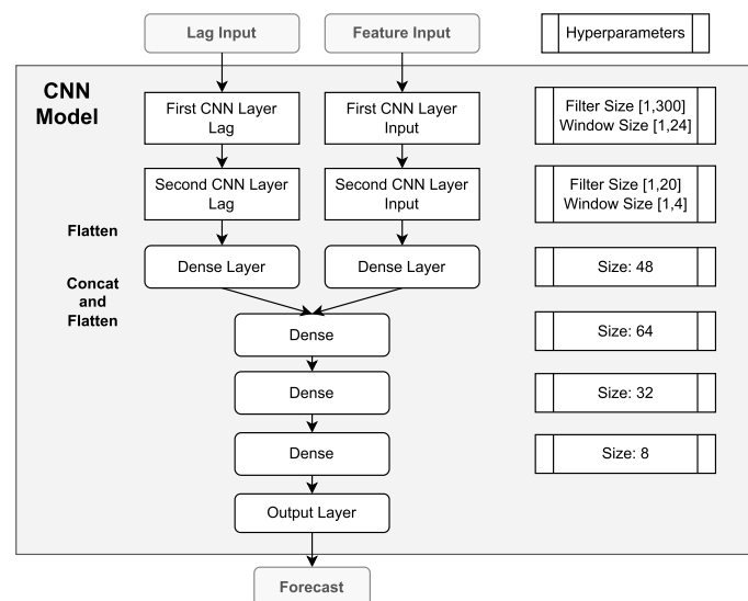
Fig. 4 The architecture of the complex CNN model used for net load forecasting. The model takes two inputs, lagged features and non-lagged features for the upcoming 24 h. The hyperparameter space used for hyperparameter optimisation is shown on the right
