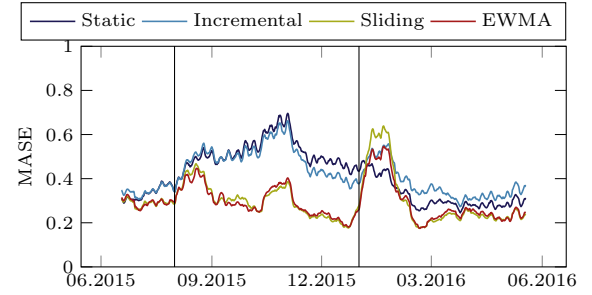
(a) The MASE of our method with different profiles on the concept drift Sudden 1.
