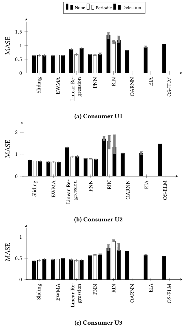
Figure 9: The MASE of our method with the EWMA and Sliding profiles and the benchmarks on the three consumers with the Incremental 1 concept drift at Position 1 for the three retraining strategies. The bars indicate the average MASE. The errors bars show the worst and the best achieved MASE of the corresponding model.
