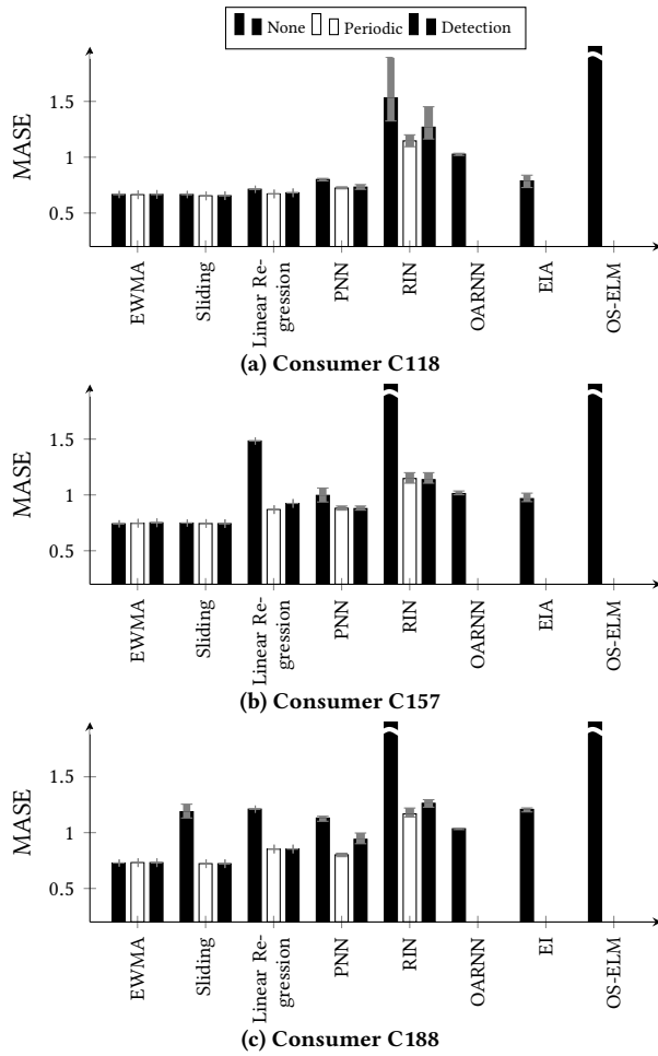
Figure 7: The MASE of the proposed method and benchmarks on the three consumers with the recorded incremental and sudden concept drifts. The bars indicate the average MASE. The errors bars show the worst and the best achieved MASE of the corresponding model.
