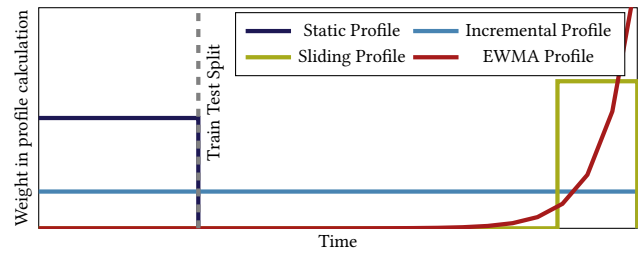
Figure 2: The four considered profile calculation methods use and weight past data differently.
