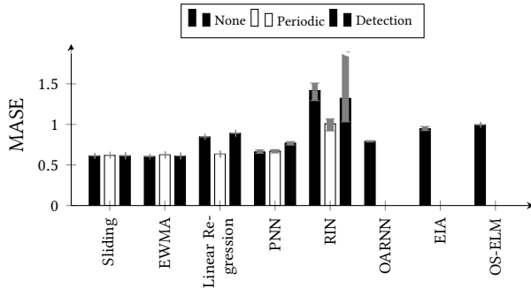
Figure 6: The MASE of our method with the EWMA and Sliding profiles and the benchmarks on consumer U1 with the Sudden 1 concept drift at Position 1 for the three retraining strategies. The bars indicate the average MASE. The errors bars show the worst and the best achieved MASE of the corresponding model.
