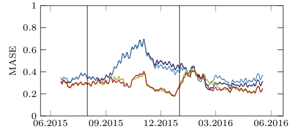
(b) The MASE of our method with different profiles on the concept drift Incremental 1.
