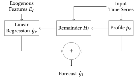
Figure 1: The proposed method for coping with concept drifts in short-term load forecasting sums a profile and a linear regression to obtain a prediction.
