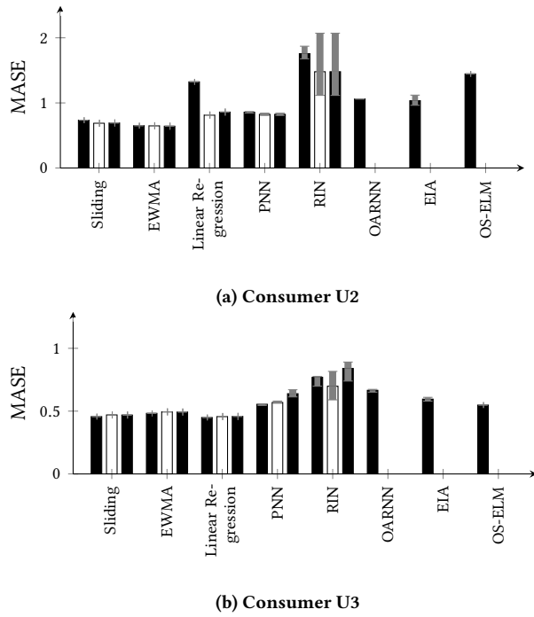
Figure 8: The MASE of our method with the EWMA and Sliding profiles and the benchmarks on the the consumers U2 and U3 with the Sudden 1 concept drift at Position 1 for the three retraining strategies. The bars indicate the average MASE. The errors bars show the worst and the best achieved MASE of the corresponding model.
