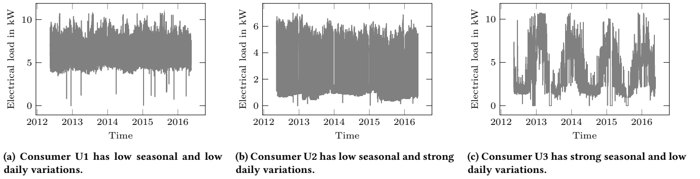
Figure 3: The three consumers from an university campus, that are used to insert synthetic concept drifts, show different seasonal and daily variations.
