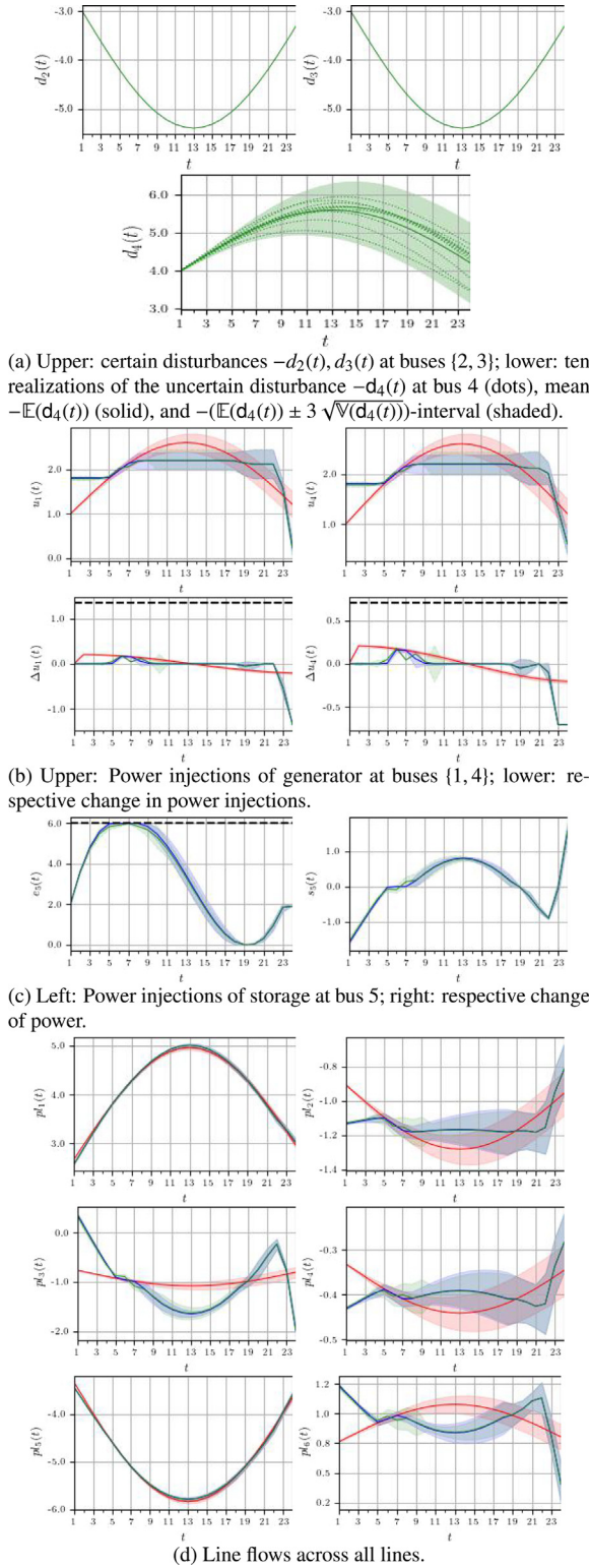
Fig. 3. IEEE 5-bus grid with artificial wind generation: Results for cases S1 (red), S2 (blue), and S3 (green). All shown random variables x are depicted in terms of their mean \mathbb{E}(x) (solid) and the interval \mathbb{E}(x) \pm \lambda(0.05)\sqrt{\mathbb{V}(x)} (shaded). (For interpretation of the references to colour in this figure legend, the reader is referred to the web version of this article.)
