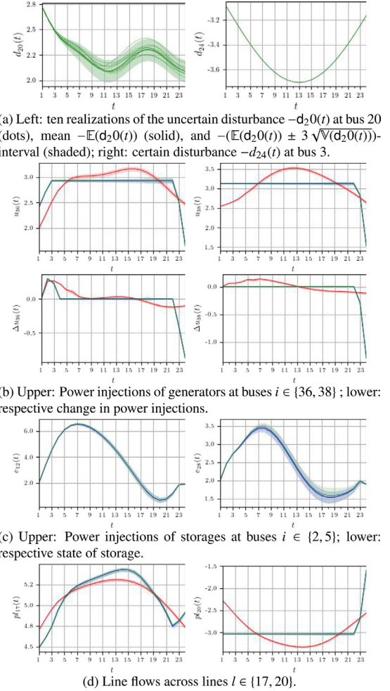
Fig. 6. IEEE 39-bus grid: Results for cases S1 (red), S2 (blue), and S3 (green). All shown random variables x are depicted in terms of their mean \mathbb{E}(x) (solid) and the interval \mathbb{E}(x) \pm \lambda(0.05)\sqrt{\mathbb{V}(x)} (shaded). (For interpretation of the references to colour in this figure legend, the reader is referred to the web version of this article.)
