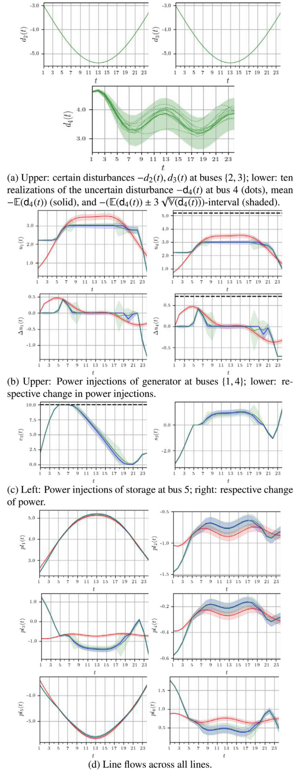
Fig. 4. IEEE 5-bus grid with real-world wind generation: Results for cases S1 (red), S2 (blue), and S3 (green). All shown random variables x are depicted in terms of their mean \mathbb{E}(x) (solid) and the interval \mathbb{E}(x) \pm \lambda(0.05)\sqrt{\mathbb{V}(x)} (shaded). (For interpretation of the references to colour in this figure legend, the reader is referred to the web version of this article.)
