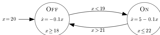
Figure 2.1: Thermostat automaton
