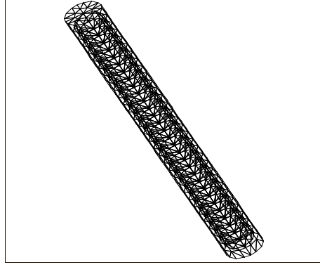
FIG. 4.4. Computational domain consisting of the cylindrical region between the mandrel and the walls of the borehole and its initial simplicial triangulation
