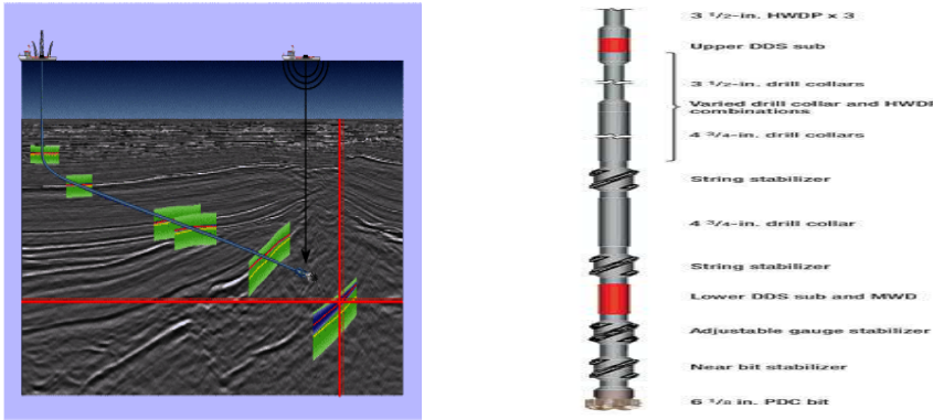
FIG. 4.1. Horizontal deepwater drilling (l.) and a typical bottomhole assembly (r.)
