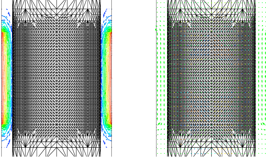
FIG. 4.6. Computed electric field (l.) and magnetic induction (r.) in a vicinity of the transmitter antenna
