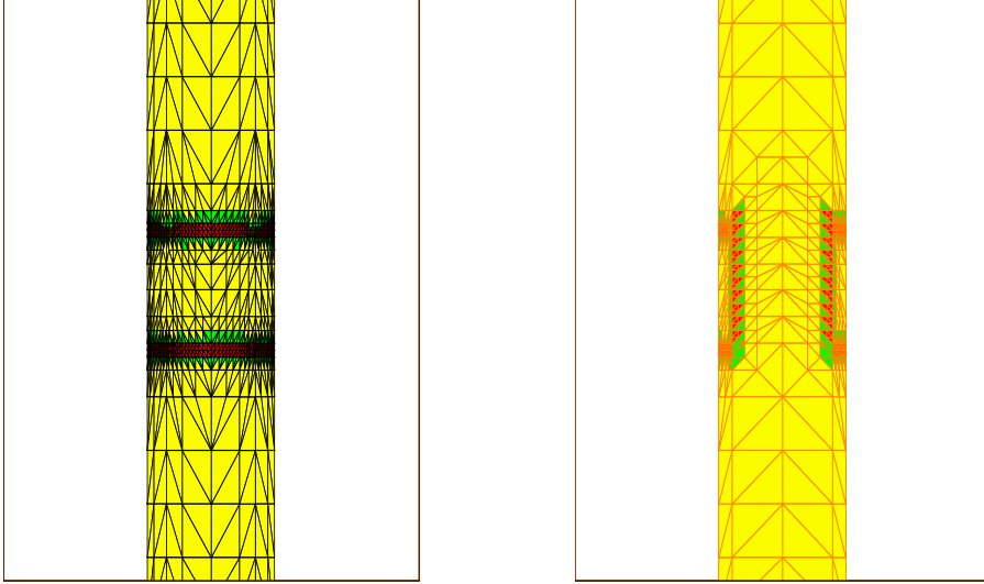
FIG. 4.5. Adaptively refined mesh on the mandrel around the coils of the transmitter antenna (l.) and around the aperture (r.)
