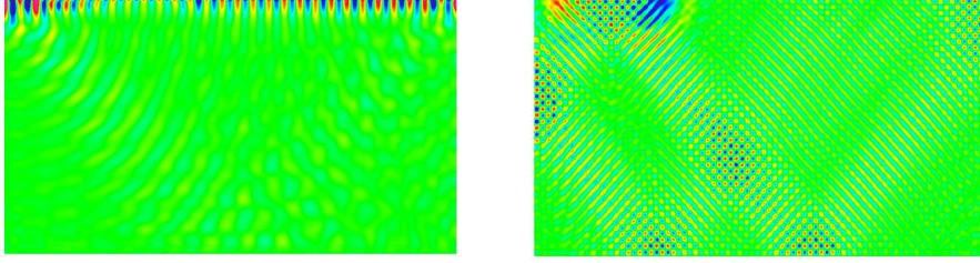
FIG. 5.1. Amplitudes of a surface acoustic wave (100 MHz) (l.) and bulk wave (200 MHz) (r.)
