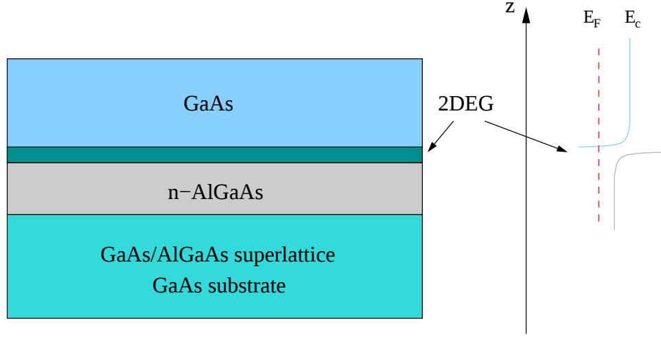
Figure 3.1: Scheme of a modulation-doped heterostructure based on the experimental setup from [51]. Of course, other types of structures exist, one popular example being the symmetric sandwich AlGaAs/GaAs/AlGaAs.
