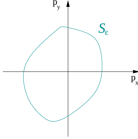
Figure F.1: A generic constant energy surface S_\epsilon parameterized by the angle \varphi , S_\epsilon = \mathbf{p}_\epsilon(\varphi) .
