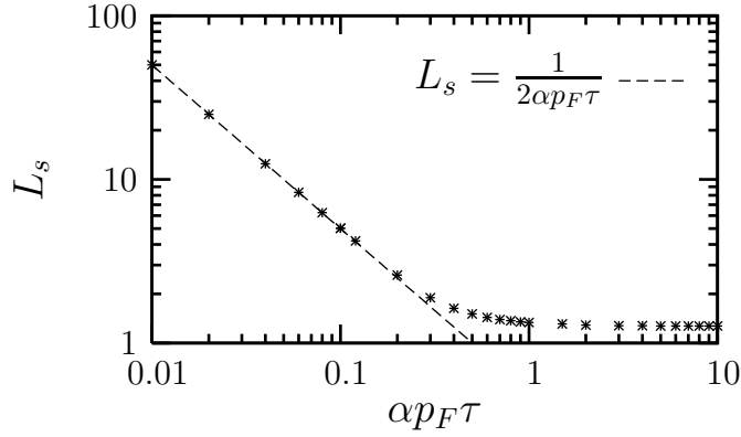
Figure 5.6: Spin relaxation length L_s in units of l as a function of disorder, obtained by fitting the spatial dependence of the electric field induced spin polarization (shown in Fig. 5.5) using s_y = a + b[\exp(-x/L_s) + \exp(-(L_x - x)/L_s)] . The diffusive limit expression is shown as a dashed line.
