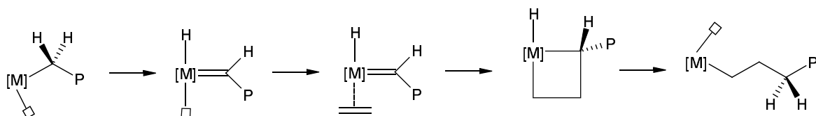
(2) Green-Rooney-Mechanismus [7]
