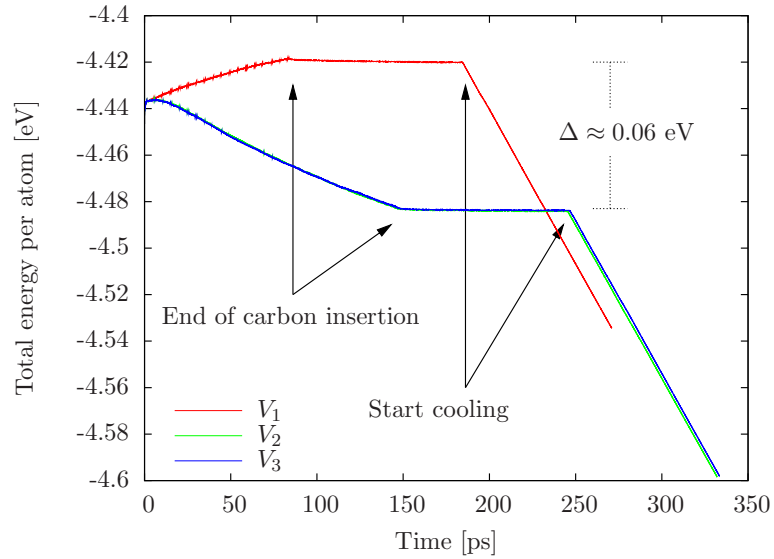
Figure 6.3: Total energy per atom as a function of time for the whole simulation sequence and for all three types of insertion volumes. Arrows mark the end of C insertion and the start of the cooling process respectively.
