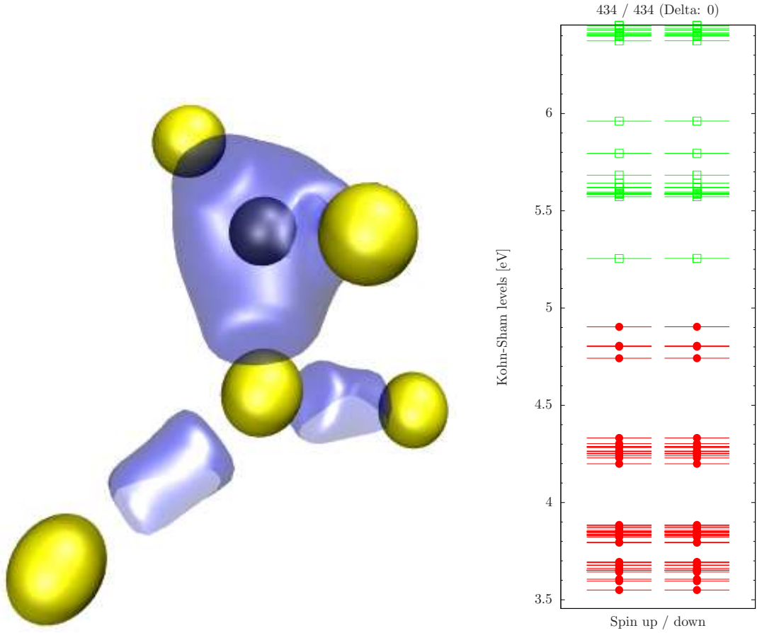
Figure 5.7: Charge density isosurface and Kohn-Sham levels of the C_i \langle 100 \rangle DB structure obtained by VASP calculations. Yellow and gray spheres correspond to Si and C atoms. The blue surface is the charge density isosurface. In the energy level diagram red and green lines and dots mark occupied and unoccupied states.
