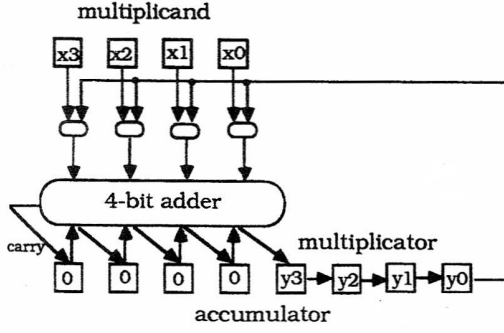
Figure 3: 4-bit serial multiplier, initial stage
