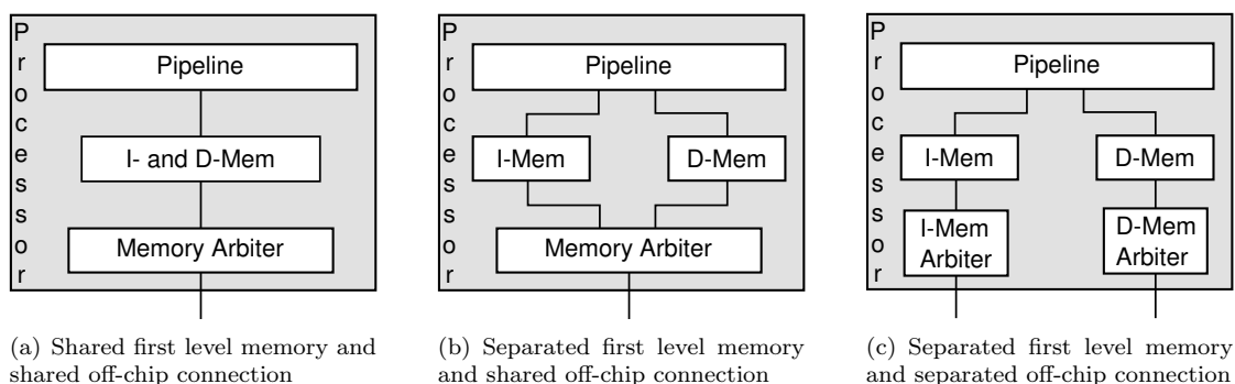
Figure 2.2: Different memory hierarchy organisations of the first level memory and the off-chip memory connection
