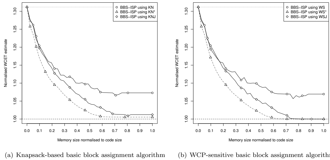
Figure A.2: Normalised WCET estimates for Compress using the BBS-ISP with the different basic block assignment algorithms
