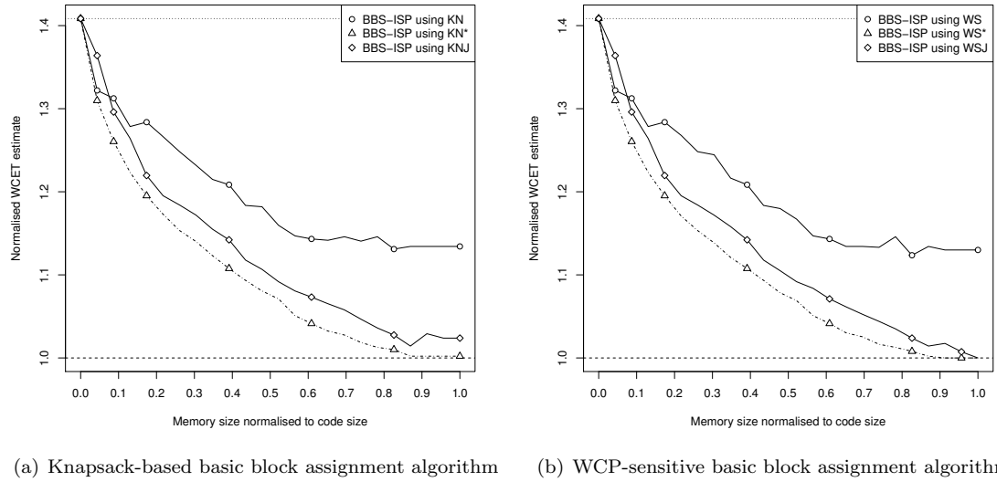
Figure A.10: Normalised WCET estimates for Rspeed using the BBS-ISP with the different basic block assignment algorithms
