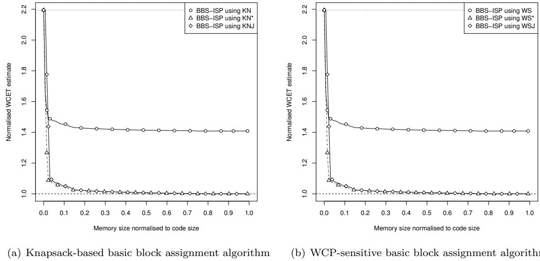
Figure A.14: Normalised WCET estimates for Ttsprk Loop using the BBS-ISP with the different basic block assignment algorithms
