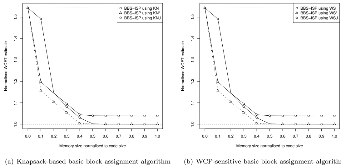
Figure A.6: Normalised WCET estimates for Matmult using the BBS-ISP with the different basic block assignment algorithms
