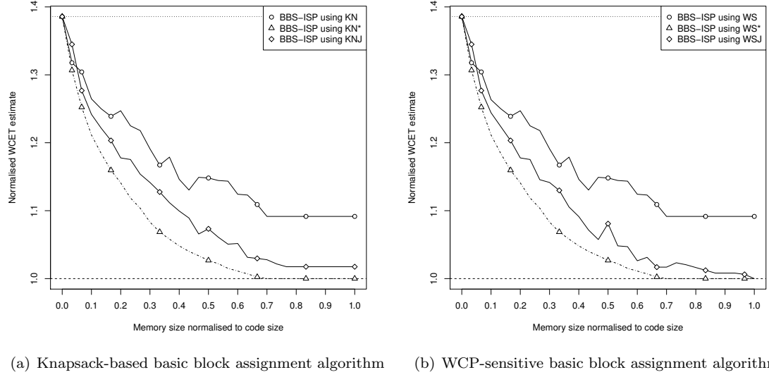
Figure A.9: Normalised WCET estimates for Puwmod Split using the BBS-ISP with the different basic block assignment algorithms
