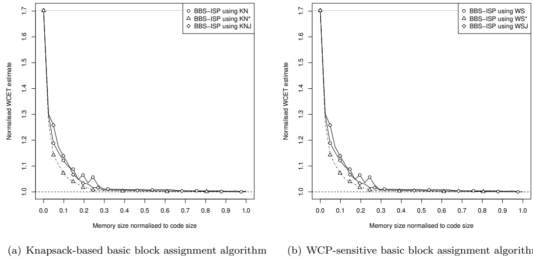
Figure A.5: Normalised WCET estimates for Edn Loop using the BBS-ISP with the different basic block assignment algorithms
