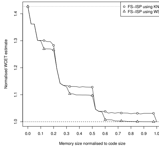
Figure A.27: Normalised WCET estimates for Sha using the FS-ISP with the different function assignment algorithms
