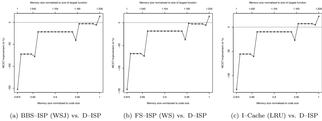
Figure 6.17: Ttsprk WCET comparison for D-ISP vs. BBS-ISP, FS-ISP, and I-Cache
