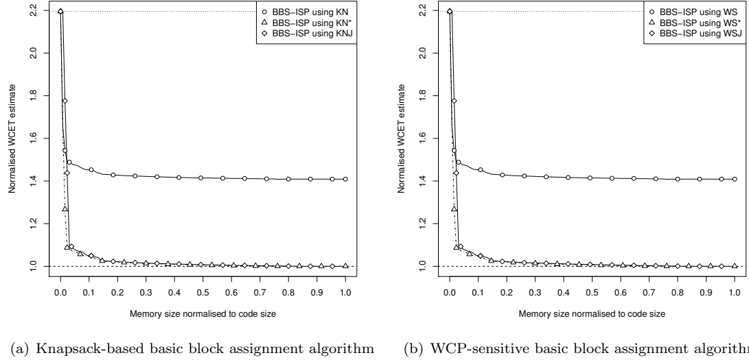
Figure A.13: Normalised WCET estimates for Ttsprk using the BBS-ISP with the different basic block assignment algorithms
