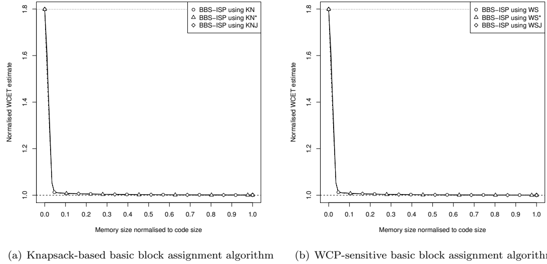
Figure A.1: Normalised WCET estimates for Adpcm using the BBS-ISP with the different basic block assignment algorithms
