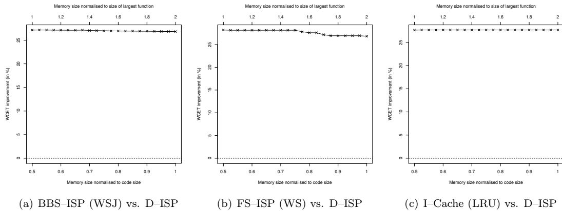
Figure 6.10: Edn WCET comparison for D-ISP vs. BBS-ISP, FS-ISP, and I-Cache
