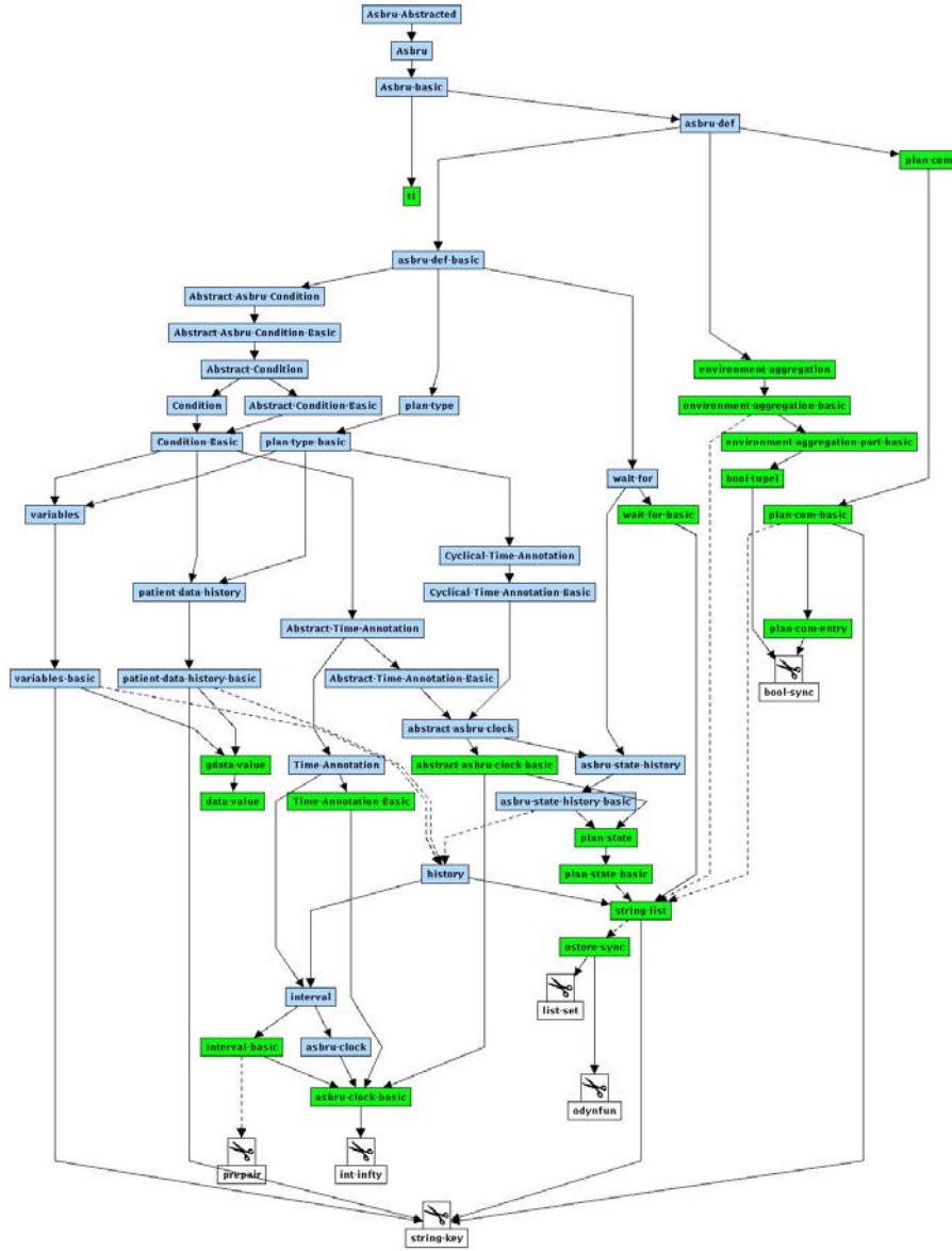
Figure 1: Asbru specification in KIV
