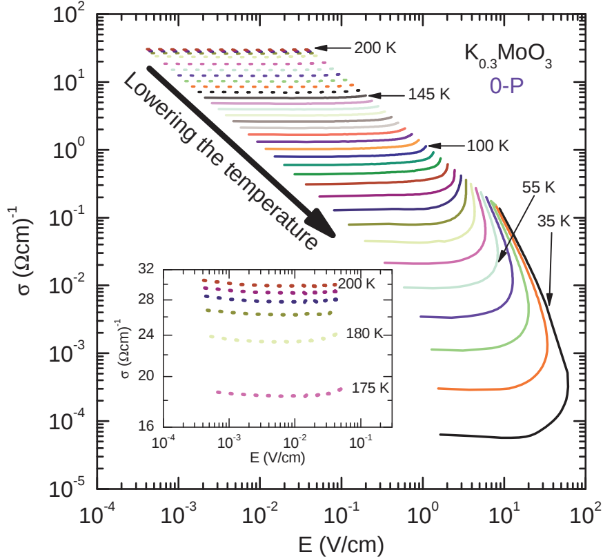
Figure 4.27: The electric field-dependent conductivity at different temperatures of K_{0.3}MoO_3 for the 0-P path.
