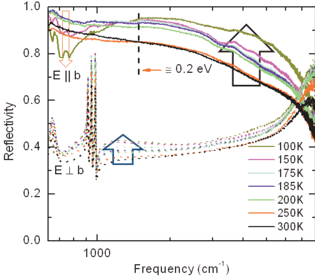
Figure 4.42: The optical reflectivity spectra parallel and perpendicular to the chain axis of a large single crystal of \text{K}_{0.3}\text{MoO}_3 . The measurements have been done using the reflection unit along with the cold finger cryostat, explained in the experiments chapter at different temperatures in the Mid-IR range.
