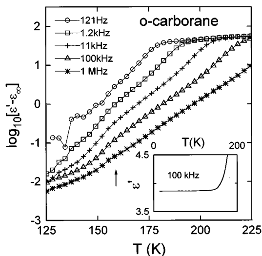
FIG. 3. Temperature dependence of the dielectric constant, \epsilon' , subtracted by the high-frequency/low-temperature limit of the dielectric constant, \epsilon_\infty . \epsilon_\infty has been determined by extrapolation of each curve to low temperatures. The arrow indicates the anomaly near 160 K. The lines connect the data points. The inset shows the temperature dependence of \epsilon' for 100 kHz at temperatures down to 12 K.
