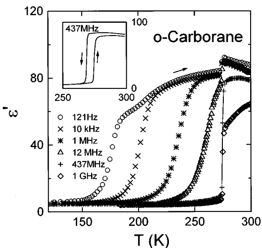
FIG. 1. Temperature dependence of the dielectric constant, \epsilon' , for various measuring frequencies as obtained on heating. The inset shows the heating and cooling curves near T_c for 437 MHz.
