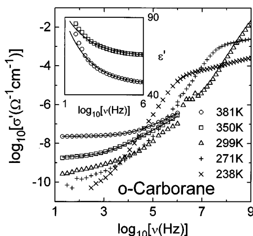
FIG. 7. Frequency dependence of the real part of the conductivity, \sigma' , for various temperatures above 238 K. The inset shows the frequency dependence of the dielectric constant, \epsilon' , for 350 and 381 K. The lines are the results of fits using the UDR, performed simultaneously on \sigma'(\nu) and \epsilon'(\nu) .
