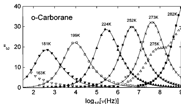
FIG. 4. Frequency dependence of the loss, \epsilon'' , for various temperatures. The lines are the results of fits using the Fourier transform of the KWW function.
