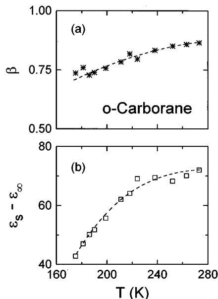
FIG. 6. Temperature dependence of the stretching parameter \beta (a) and of the relaxation strength \epsilon_s - \epsilon_\infty (b) as obtained from fits of \epsilon''(\nu) using the Fourier transform of the KWW function. The lines are drawn to guide the eyes.
