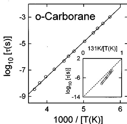
FIG. 5. Temperature dependence (Arrhenius representation) of the relaxation time \tau_{\text{KWW}} as obtained from fits of \epsilon''(\nu) with the Fourier transform of the KWW function. The solid line is the result of a fit using the Arrhenius law. The inset demonstrates the deviations of the relaxation times of ortho -carborane from maximal strong behavior (dashed line).
