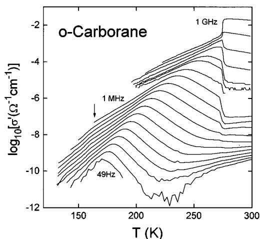
FIG. 2. Temperature dependence of the real part of the conductivity, \sigma' , for various frequencies. The frequencies are (from top to bottom): 1 GHz, 331 MHz, 110 MHz, 36 MHz, 12 MHz, 6.9 MHz, 2.3 MHz, 1 MHz, 499 kHz, 167 kHz, 67 kHz, 27 kHz, 4.5 kHz, 1.9 kHz, 735 Hz, 299 Hz, 121 Hz, and 49 Hz. The arrow indicates the anomaly near 160 K.
