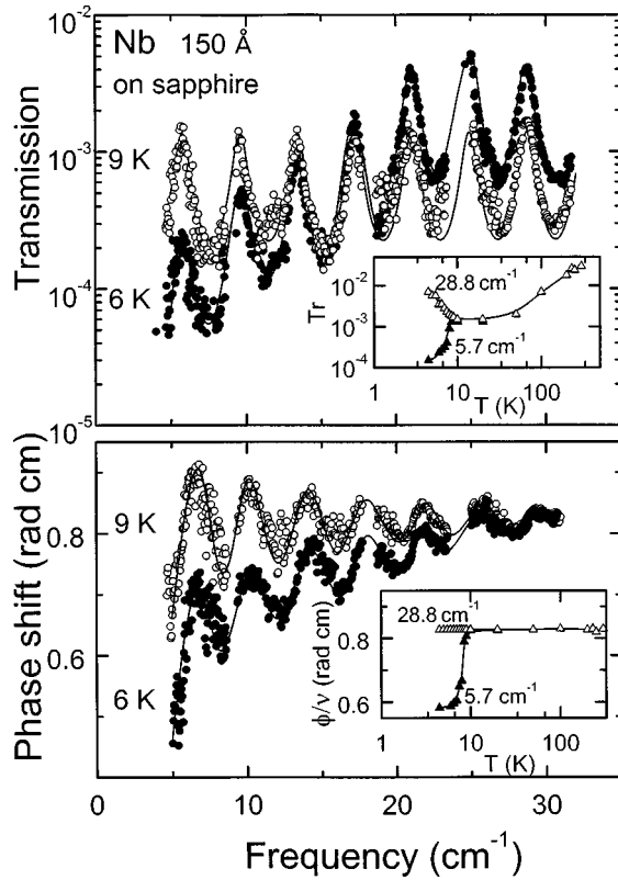
FIG. 3. Original transmission Tr(\nu) and phase shift \varphi(\nu) spectra of the Nb film on the Al_2O_3 substrate. The phase shift is divided by the frequency for the better perception. The dots represent the measured values, the lines for 9 K are the fit with the Drude model. In the insets the temperature dependence of Tr and \varphi is displayed for two particular frequencies corresponding to the first and last transmission maxima in our spectral range.
