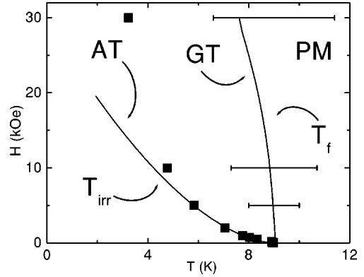
FIG. 4. Magnetic-field dependent phase diagram of \text{Li}_{0.8}\text{Zn}_{0.2}\text{V}_2\text{O}_4 , where the lines are the AT and GT lines and PM the paramagnetic phase. T_{irr} and T_f are used as defined in the text.
