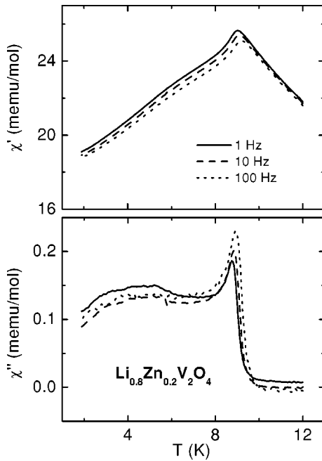
FIG. 6. Real (upper panel) and imaginary (lower panel) part of the ac susceptibility of \text{Li}_{0.8}\text{Zn}_{0.2}\text{V}_2\text{O}_4 at frequencies of 1, 10, and 100 Hz vs temperature between 1.9 and 12 K.
