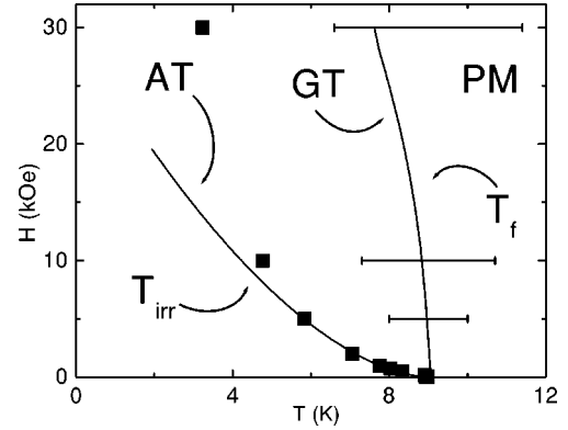
FIG. 4. Magnetic-field dependent phase diagram of \text{Li}_{0.8}\text{Zn}_{0.2}\text{V}_2\text{O}_4 , where the lines are the AT and GT lines and PM the paramagnetic phase. T_{irr} and T_f are used as defined in the text.
