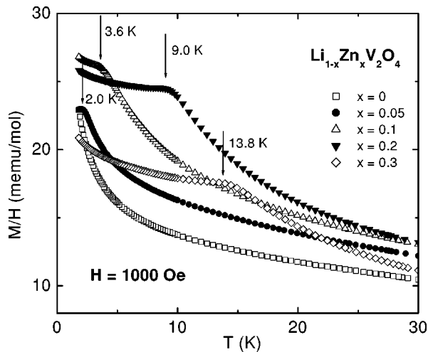
FIG. 1. Temperature-dependent magnetization divided by the applied field of 1000 Oe in \text{Li}_{1-x}\text{Zn}_x\text{V}_2\text{O}_4 between 1.9 and 30 K for x=0, 0.05, 0.1, 0.2, and 0.3 and temperatures 1.9 \leq T \leq 30 K. Arrows indicate the spin-glass temperatures T_f , as derived from \chi'_{ac} .
