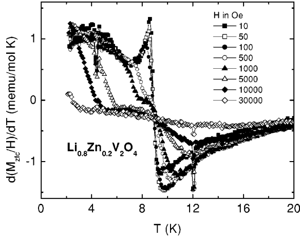
FIG. 3. Temperature derivative of the zero-field-cooled magnetizations divided by the applied field of \text{Li}_{0.8}\text{Zn}_{0.2}\text{V}_2\text{O}_4 for applied fields of 10, 50, 100, 500, 1000, 5000, 10 000, and 30 000 Oe vs temperature between 1.9 and 20 K.
