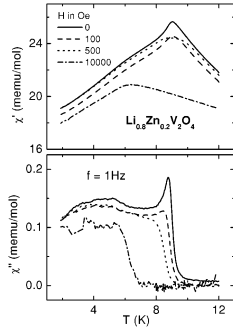
FIG. 7. Real (upper panel) and imaginary (lower panel) part of the ac susceptibility of \text{Li}_{0.8}\text{Zn}_{0.2}\text{V}_2\text{O}_4 at 1 Hz for applied dc fields of 0, 100, 500, and 10 000 Oe vs temperature between 1.9 and 12 K.
