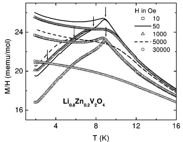
FIG. 2. Zero-field-cooled (lower curves) and field-cooled (upper curves) magnetization divided by the applied field H vs temperature for \text{Li}_{0.8}\text{Zn}_{0.2}\text{V}_2\text{O}_4 between 1.9 and 16 K for applied fields of 10, 50, 1000, 5000, and 30 000 Oe. Arrows indicate the temperature T_{irr} where the FC and ZFC curves split.
