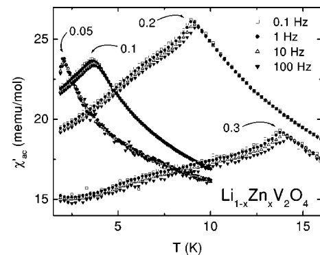
FIG. 5. Temperature dependence of the ac susceptibility of \text{Li}_{1-x}\text{Zn}_x\text{V}_2\text{O}_4 for x=0.05, 0.1, 0.2, 0.3 at different frequencies.
