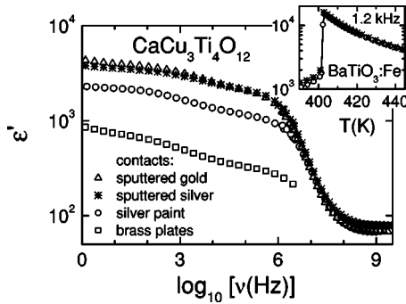
FIG. 3. Frequency-dependent dielectric constant at room temperature of a CCTO sample, successively prepared with different contact types. The inset shows \epsilon'(T) of Fe-doped ferroelectric BaTiO 3 close to T_c , measured with silver paint and sputtered silver contacts.
