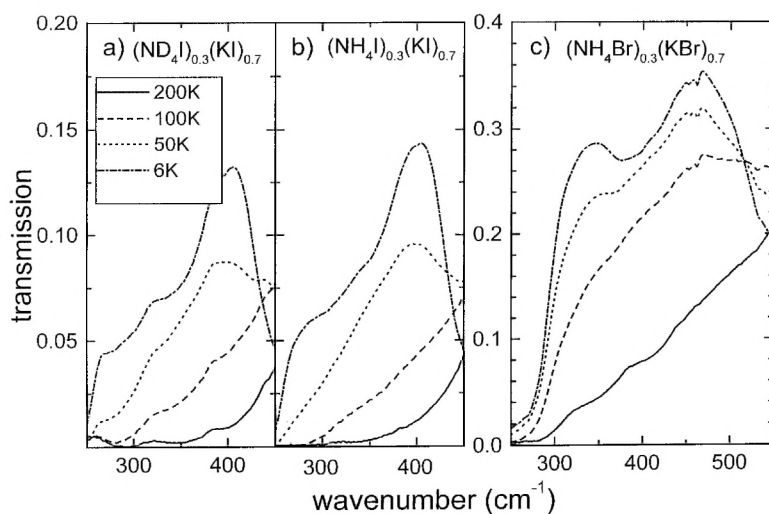
Figure 2. The FIR transmission spectra of (a) (ND 4 I) 0.3 (KI) 0.7 , (b) (NH 4 I) 0.3 (KI) 0.7 and (c) (NH 4 Br) 0.3 (KBr) 0.7 for temperatures between T = 6 K and T = 200 K. Note the different frequency scale in (c).
