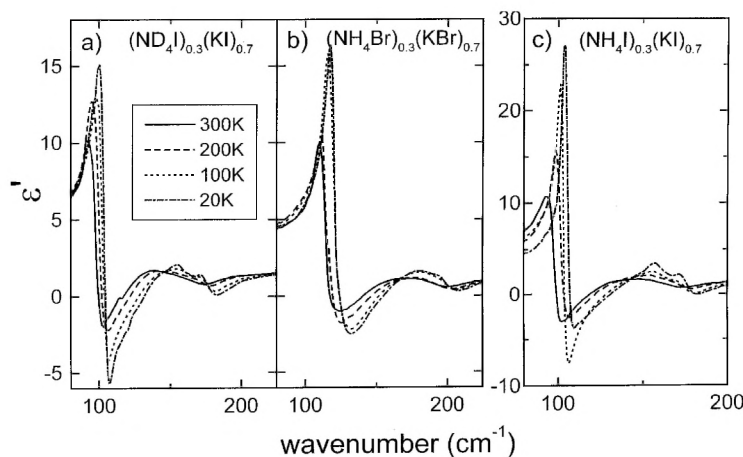
Figure 3. Frequency dependence of the dielectric constant \epsilon' for temperatures between 20 K and 300 K in (a) (ND 4 I) 0.3 (KI) 0.7 , (b) (NH 4 Br) 0.3 (KBr) 0.7 and (c) (NH 4 I) 0.3 (KI) 0.7 . For reasons of representation the bromide compound is shown in (b).
