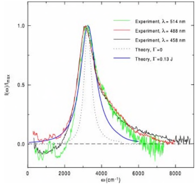
FIG. 2. Comparison of the theoretical result without ( \Gamma = 0 ) and with additional damping ( \Gamma = 0.13J ) to the experimental Raman intensity in \text{La}_2\text{CuO}_4 in B_{1g} geometry taken from Ref. 3. Calculations were performed with the parameter set (16). The three experimental curves belong to different incoming photon frequencies; the high-energy intensity background was subtracted. All datasets were normalized to their corresponding intensity maximum.
