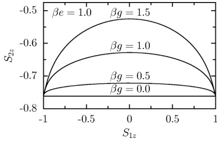
FIG. 2. The Bloch vector component S_{z2} as a function of S_{z1} resulting from Eq. (28) for \beta e = 1 and different values \beta g = 0, 0.5, 1, 1.5 . Note that a strictly linear dependence results only for the case of vanishing coupling g = 0 . An approximate linear regime exists in a neighborhood of S_{1z} = 0 .
