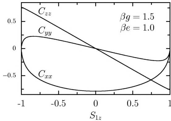
FIG. 3. The nonvanishing correlation functions C_{xx}, C_{yy}, C_{zz} as a function of the Bloch vector component S_z for \beta e = 1 and \beta g = 1.5 . The correlation functions C_{xx} and C_{yy} clearly deviate from straight lines following from a convex blow-up map, see Eq. (31). For the correlation functions also an approximately linear regime exists in a neighborhood of S_{1z} = 0 .
