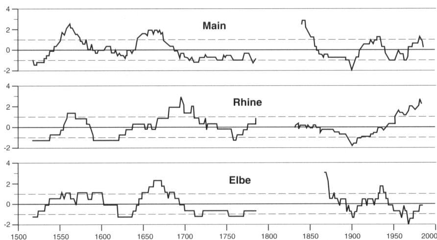
Fig. 6: 31-year running mean values of the winter flood frequencies for the three larger central European rivers Main, Rhine and Elbe
