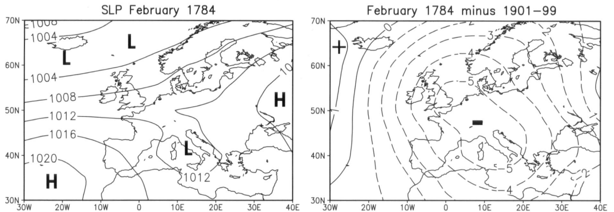
Fig. 5: Representation of the reconstructed mean SLP field for February 1784 (LUTERBACHER et al. 2002), a month whose synoptic configuration was responsible for one of the most severe flood catastrophes in central Europe in the last centuries (see Fig. 2a). a) monthly mean surface pressure, contours of the isobars at 4 hPa intervals. b) anomaly pattern (February 1784 minus February 1901–1999), contour intervals at 1 hPa
