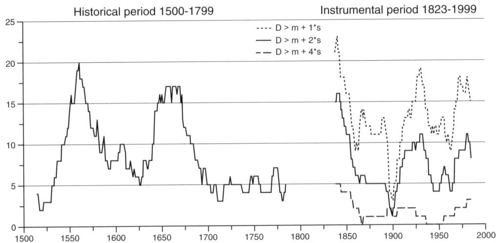
Fig. 4: 31-year running frequencies of winter flooding events in the Main River area for the pre-instrumental period from 1500 to 1799 (left) and of extreme discharge rates at the Würzburg gauge for the instrumental period from 1823 to 1999 (right; see the explanations concerning the different thresholds in the upper right hand corner). D: monthly maximum discharge / m: mean of monthly maximum discharges / s: standard deviation of monthly maximum discharges
