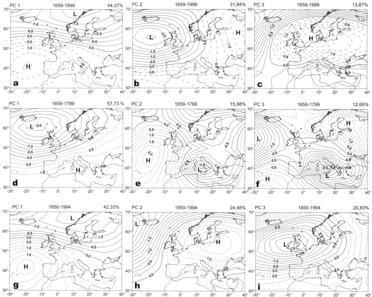
Fig. 8: SLP patterns of the first three PCs of monthly mean SLP grids during winter months: a–c) for all SLP grids between 1659 and 1999; d–f) for the winter months with flood events at the rivers Main, Rhine, Elbe or Weser between 1659 and 1799 (pre-instrumental period); g–i) like d–f, but for 1850–1994 (instrumental period)
