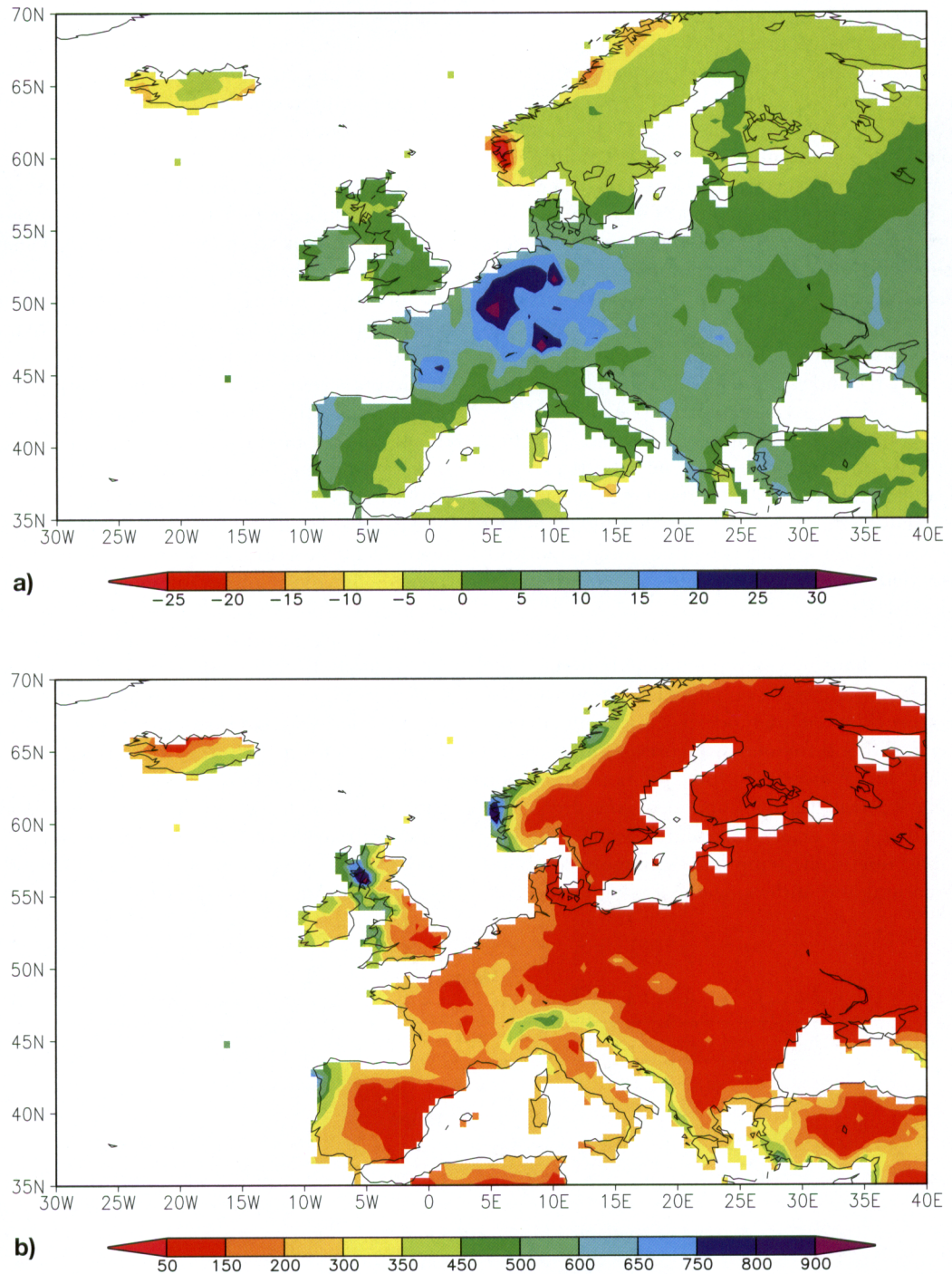
Fig. 7: Reconstructed European precipitation patterns: a) Composite of precipitation anomalies (mm per month) of 20 winter months with strong winter flooding in at least one of the three central European river catchments between 1784 and 1995, related to the 1961–1990 mean. b) Reconstructed average winter precipitation (mm) for continental Europe between 1784 and 1995
