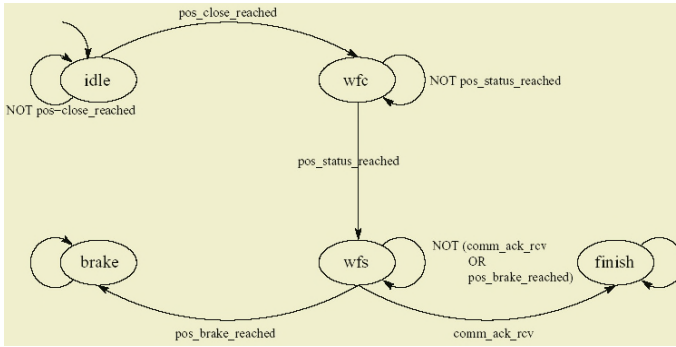
Fig. 7. Model of the train control
