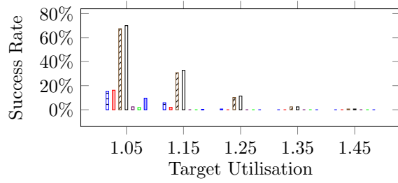
Figure A.10.: Performance with restricted m_i ( r_m = 0.6 ) and realistic periods
