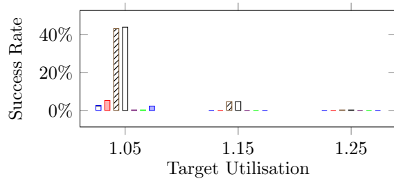
Figure A.12.: Performance with restricted m_i ( r_m = 0.8 ) and realistic periods
