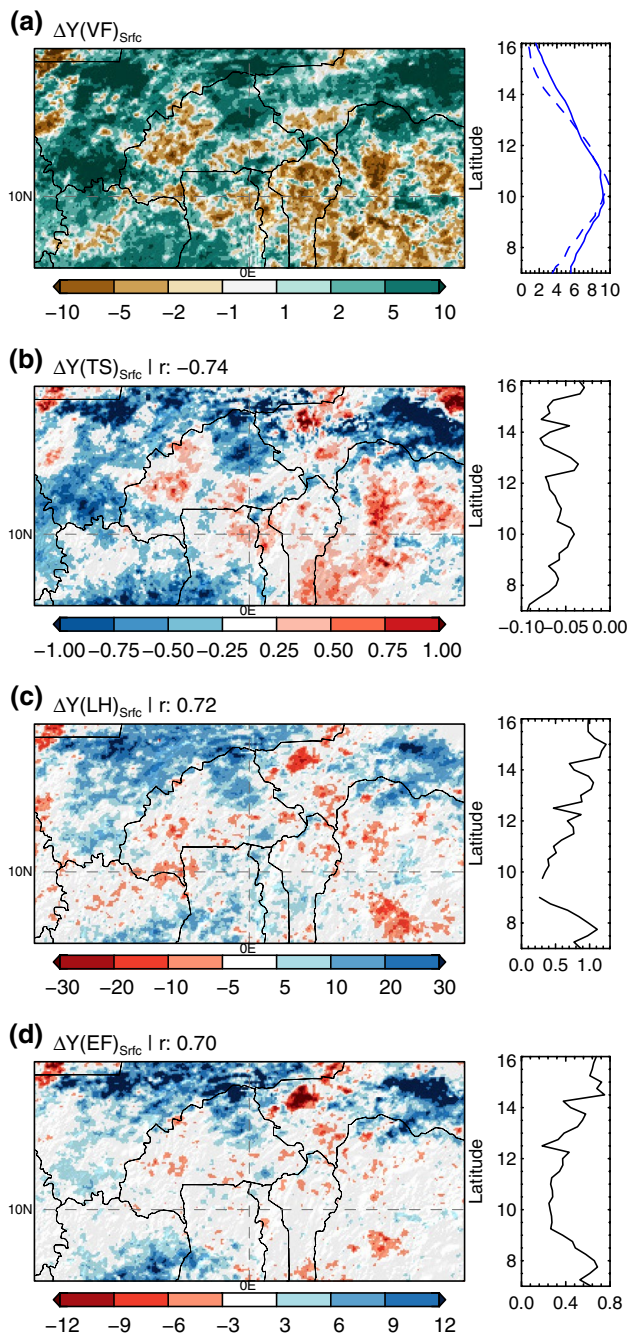
Fig. 8 Left Aug–Sep maps of \Delta Y_{Srfc} for a vegetation fraction (VF, %), b surface temperature (TS, K), c latent heat flux (LH, W m^{-2} ) and d evaporative fraction (EF, %). EF is defined as the ratio of latent heat flux to the sum of latent and sensible heat fluxes. Spatial correlations ( r ) are with respect to \Delta Y(VF)_{Srfc} . Only significant \Delta Y_{Srfc} are shown ( P \leq 0.01 ) and taken into account to compute r . Right a the meridional average precipitation ( mm day^{-1} , 2010: solid, 2009: dashed) and b–d the coefficients a (the slope) of the zonal slices linear fit ( ax+b ) between \Delta Y(VF)_{Srfc} and \Delta Y(TS)_{Srfc} , \Delta Y(LH)_{Srfc} and \Delta Y(EF)_{Srfc} , respectively. Missing values indicate no correlation for the zonal slice
