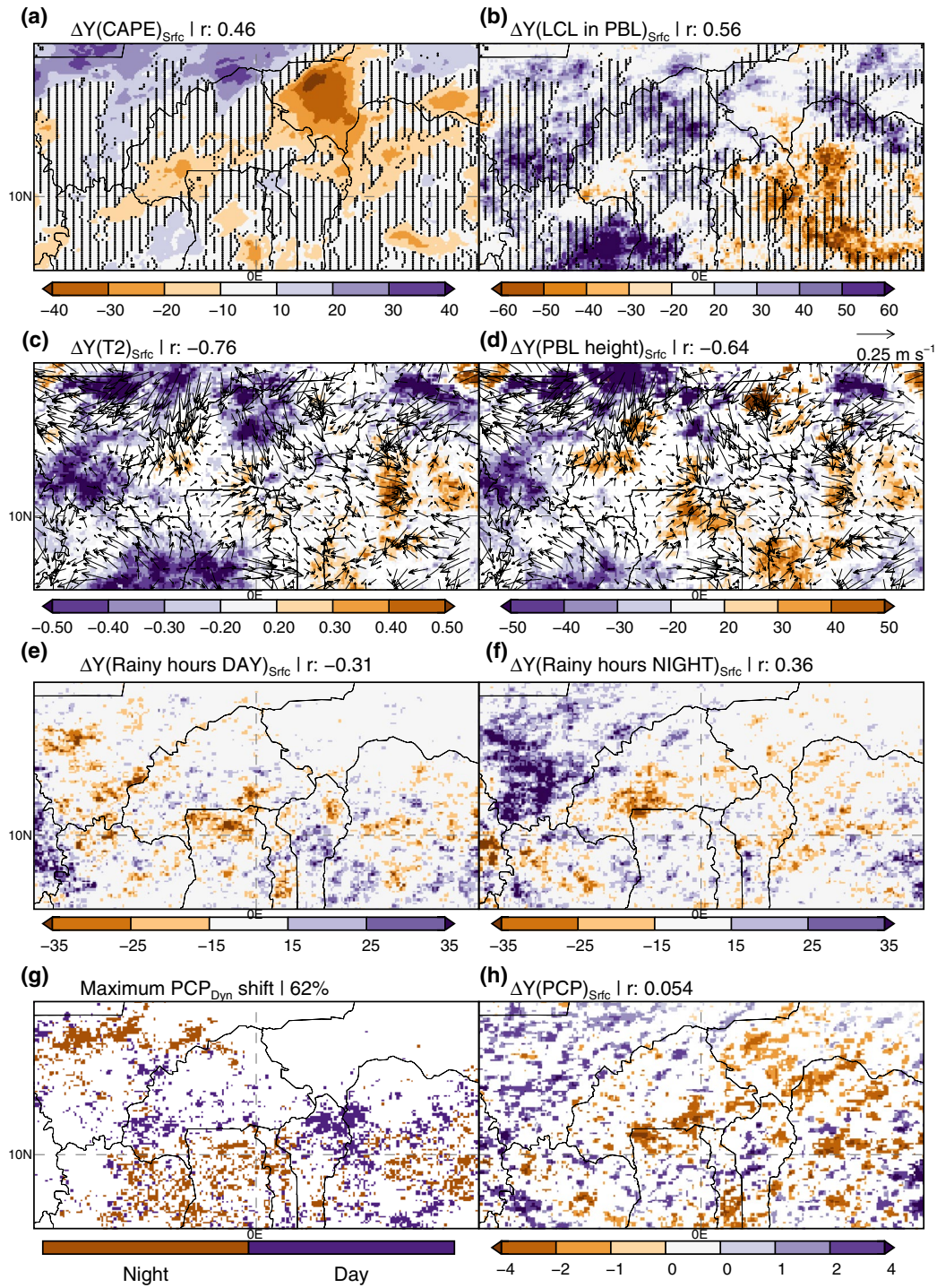
Fig. 10 Maps for Aug–Sep: a \Delta Y(CAPE)_{Srfc} (J kg -1 ), b \Delta Y_{Srfc} for the number of daytime hours in which the PBL height reaches the lifted condensation level (LCL). Stripes in a , b mark insignificant changes of CAPE. c , d \Delta Y_{Srfc} for 2m temperature (T2, K), PBL height (m) and 10 m wind vectors (m s -1 ). (e,f) \Delta Y_{Srfc} of rainy hours during the day (0700–1800 UTC)/ night ( \geq 1 mm h -1 ), g pixels showing a shift of the precipitation maximum from night to day (“Day”
