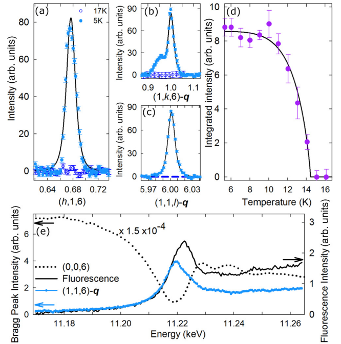
FIG. 1. Magnetic peak at (1, 1, 6) - \mathbf{q} . (a)–(c) Scans along three different reciprocal space directions (filled/open symbols are at base temperature/above T_N ). Solid lines are fits to a Lorentzian-squared shape [panel (b) shows a side shoulder attributed to the finite sample mosaic]. (d) Temperature dependence of the integrated peak intensity (solid line is guide to the eye). (e) Energy scan through the magnetic peak (thick blue solid symbols) showing a large resonant enhancement with a maximum at the onset edge of the fluorescence signal from the sample (black solid line, scaled). In contrast, the same energy scan through a structural peak (dotted line) shows minimum intensity near resonance (due to increased x-ray absorption). Data points in all panels are shown with an estimate of the incoherent background subtracted off.
