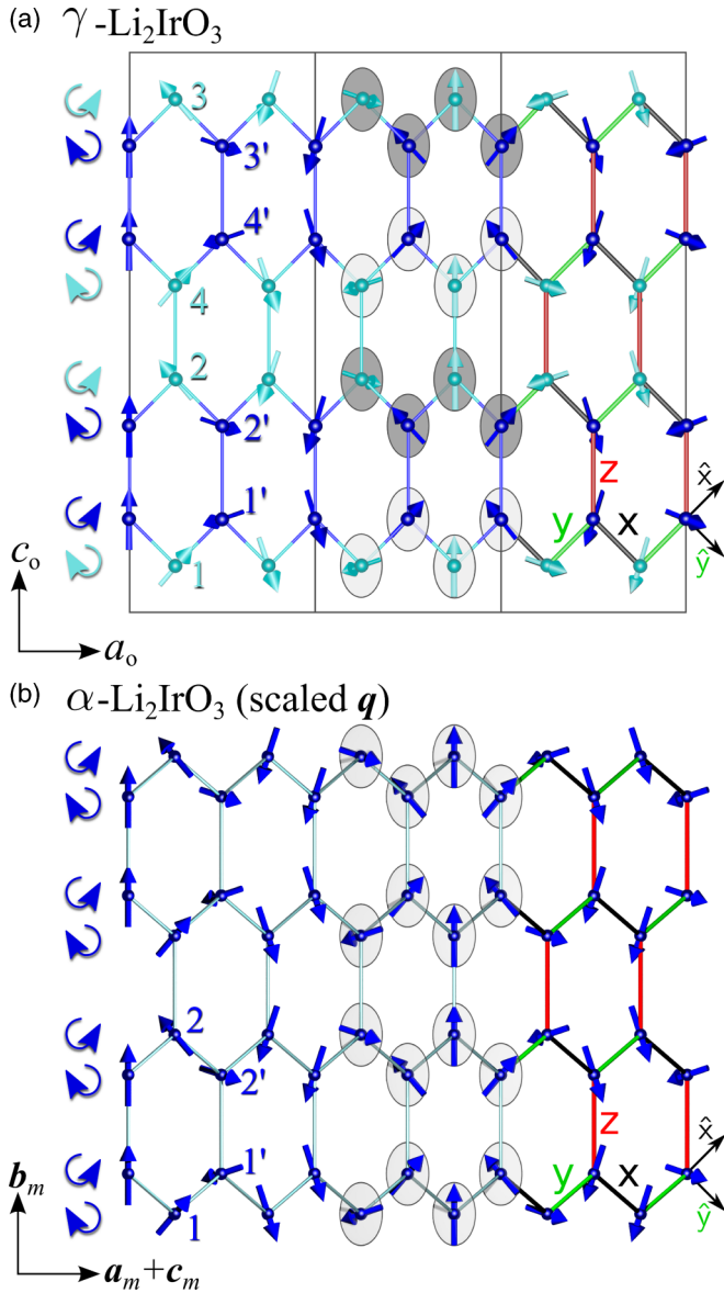
FIG. 7. (a) Magnetic structure in \gamma - \text{Li}_2\text{IrO}_3 projected onto the orthorhombic a_o c_o plane (from Ref. [16]). (b) For comparison, the magnetic structure in one honeycomb layer of \alpha - \text{Li}_2\text{IrO}_3 is plotted for a scaled propagation vector, f\mathbf{q} , with f = 0.89 , such that it shows the same periodicity of moment rotation as in \gamma - \text{Li}_2\text{IrO}_3 . For both structures left curly arrows indicate counterrotation of moments between consecutive sites along c_o and both magnetic structures are plotted for three orthorhombic cells along the horizontal direction. In (a) light/dark shaded elliptical envelopes in unit cell 2 illustrate the alternation of the orientation of the plane of rotation between adjacent vertically stacked zigzag chains, whereas no such alternation occurs in the \alpha magnetic structure [panel (b)]. In unit cell 3 the color of bonds indicates the anisotropy axis of Kitaev exchange with black/green/red for x,y,z. The Kitaev axes are normal to the Ir-O 2 -Ir bond planes and are shown by the unit vectors \hat{x}, \hat{y} ( \hat{z} into the page), as defined in Eq. (B2). In (b) the axes labels a_m, b_m , and c_m indicate the “symmetrized” monoclinic axes defined in Eq. (B1).
