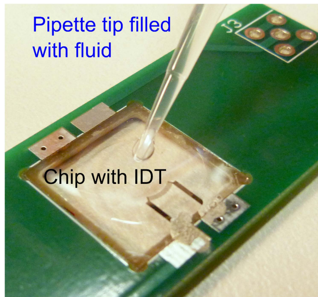
Figure 1. Experimental set-up, where the transparent \text{LiNbO}_3 chip is shown with a focusing IDT mounted on a circuit board (green). The chip is wetted with a liquid (in this case isopropanol) creating a thin fluid film covering the chip.
