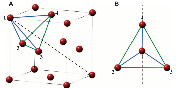
Fig. 6. Bond symmetry in the rhombohedrally distorted structure of GaV 4 S 8 . (A) V 4 clusters (red spheres) form an fcc lattice that is stretched along one of the body diagonals (dashed line). Two types of bonds result from this distortion, as illustrated for four selected clusters: intraplane bonds (green lines) between nearest-neighbor V 4 units within the (111) planes and interplane bonds (blue lines) connecting V 4 units in neighboring (111) planes. (B) The four selected clusters viewed from the \langle 111 \rangle direction. Each blue bond lies within a mirror plane of the tetrahedron (see dashed line for an example), whereas green bonds are perpendicular to them.
