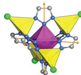
Fig. 1 Kuratowski-type SBU of MFU-4-type frameworks (central octahedrally coordinated metal ion: purple octahedron, peripheral Zn: yellow tetrahedra; N: blue; C: grey, Cl: green).
