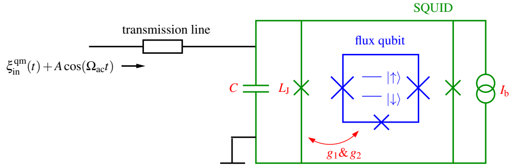
Figure 1. Sketch of the flux qubit (blue) coupled to a dc SQUID. The interaction is characterized by the linear coupling g_1 , which depends linearly on the SQUID bias current I_b and the quadratic coupling g_2 . The SQUID with Josephson inductance L_J is shunted by a capacitance C . The frequency shift of the resulting harmonic oscillator (green) can be probed by external resonant ac excitation A \cos(\Omega_{ac} t) via the transmission line (black), in which the quantum fluctuations \xi_{in}^{qm}(t) are also present.
