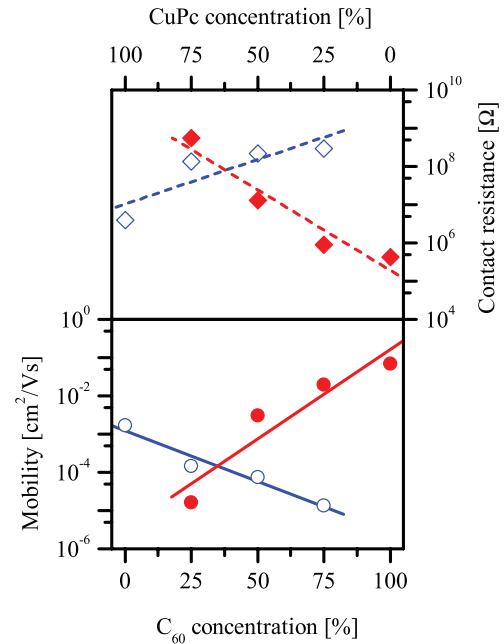
Figure 5. Contact resistance and mobility versus concentration in CuPc:C 60 mixtures for the SCA (left) and the analysis using TLM (right). The effective gate voltage |V_G - V_T| is 30 V (open symbols: hole transport and filled symbols: electron transport).
