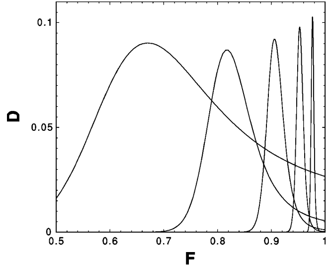
FIG. 4. Diffusion coefficient (22) versus the tilt F for a potential V(x) defined via Eqs. (25),(26) with q = 3/2 for all x \in [-L/2, L/2] while outside [-L/2, L/2] it is fixed by Eqs. (2),(3). Using dimensionless units, the parameter values are \eta = 1, L = 2, \mu = 1, F_c = 1 . The five curves with increasingly sharper peaks correspond to the following five values of kT = D_0 : 3 \times 10^{-2}, 10^{-2}, 10^{-3}, 10^{-4}, and 10^{-5} . The theoretically predicted peak height for asymptotically small kT from Eq. (68) is 0.1 .
