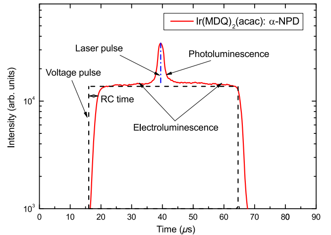
FIG. 3. Illustration of an exemplary pulse sequence performed on the red phosphorescent OLEDs. The dashed lines represent the electrical and optical excitation. The red solid line displays the measured luminescence as a reaction to both excitations. For better visual separation of the EL and PL, an electrical pulse duration of 50 \mu s is chosen for this illustration.
