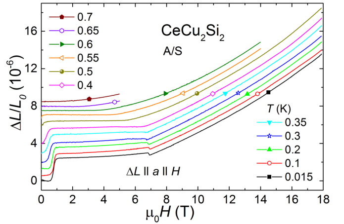
FIG. 2. Length change \Delta L/L_0 normalized to L_0 versus applied magnetic field H \parallel \Delta L \parallel a between zero and 17.9 T is shown for temperatures in the range 0.015–0.7 K. We observe clear steps at the SC transition at 1 T and around 7 T separating phase A from B for lowest temperatures. The anomaly at 1 T shifts to lower fields with increasing T , whereas the step between phase A and B is clearly visible to 0.3 K and gets less pronounced at higher temperature.
