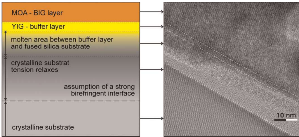
Figure 19 (online color at: www.pss-a.com ) Left side: The model developed for the simulation of the YIG buffer systems. A thin YIG layer rests in a transitional area with Y and Fe diffused into it. Right side: The TEM image of a (10\bar{1}0) sample as the base for the model stack. Molten or crystalline areas are marked.
