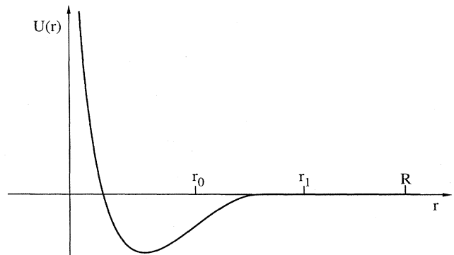
FIG. 24. Potential form used for a recombination reaction, exhibiting a short-range attracting part. Absorption takes place at r_0 and reflection at r = R , while r_1 denotes the initial separation.
