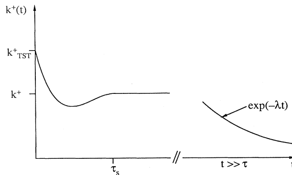
FIG. 4. Characteristic behavior of the reactive flux k^+(t) in Eq. (2.25) with \lambda \equiv k^+ + k^- . At times t < \tau_s one observes transient recrossings. The rate k^+ appears as the plateau value at long times t \gg \tau_s . At extremely long times t \sim (k^+)^{-1} , the reactive flux exhibits an exponential decay, which is not yet noticeable on the intermediate time scale \tau defined through Eq. (2.19).
