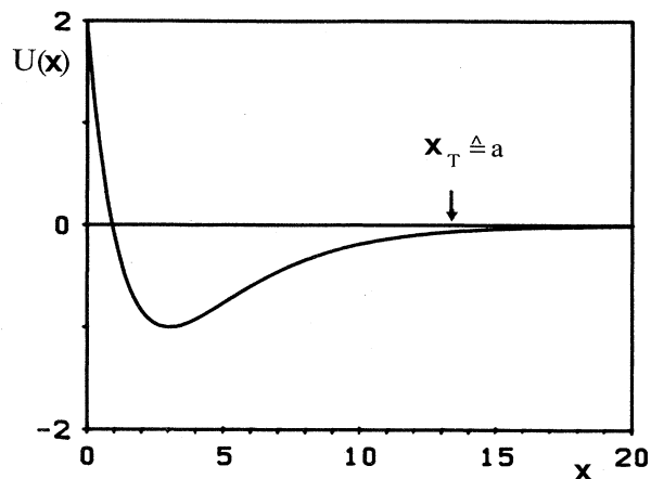
FIG. 7. The one-dimensional Morse potential U(x) = -E_D + E_D \{1 - \exp[-(x - x_s)/b]\}^2 , with E_D=1 , x_s=b=3 . The state x_T=a denotes the arbitrarily chosen transition point.
