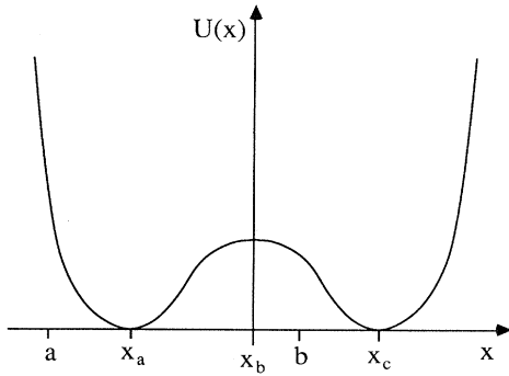
FIG. 20. Double-well potential used in text.
