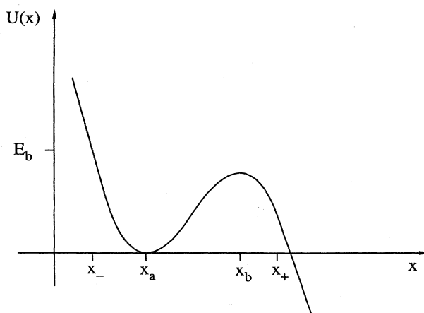
FIG. 13. Metastable potential field used in text. Particles are injected at x_- and immediately removed when they arrive at x_+ .
