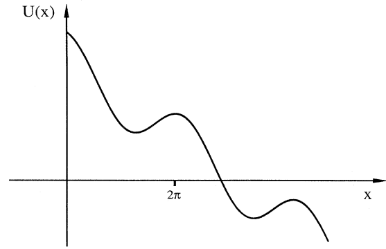
FIG. 29. Form of the biased periodic potential used in text. Note that the states x and x + 2\pi are considered distinguishable.
