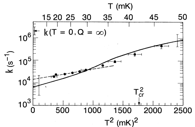
FIG. 52. Low-temperature quantum-Kramers rate data from the Berkeley experiment (Cleland, Martinis, and Clarke, 1988). The solid line is the theoretical crossover prediction of Grabert and Weiss (1984b). The vertical error bars arise from systematic errors for the parameters of the junction; the horizontal error bars indicate the uncertainty in the temperature calibration. The horizontal arrow denotes the zero-temperature, undamped quantum rate, and T_{cr}^2 denotes the squared crossover temperature, Eq. (9.14). The dashed line indicates a least-squares linear fit of the data below 30 mK to \ln k(T) = A + BT^2 . The asymptote of the data is A = 9.4 \pm 0.5 , while the theory in Eq. (9.39) predicts A = 8.8 \pm 1.0 . The slope of the T^2 law [see Eq. (9.40)] for the data is B = (1.3 \pm 0.1) (\text{mK})^{-2} , while theory yields B = (1.9 \pm 0.2) (\text{mK})^{-2} . Figure obtained from Professor Clarke.
