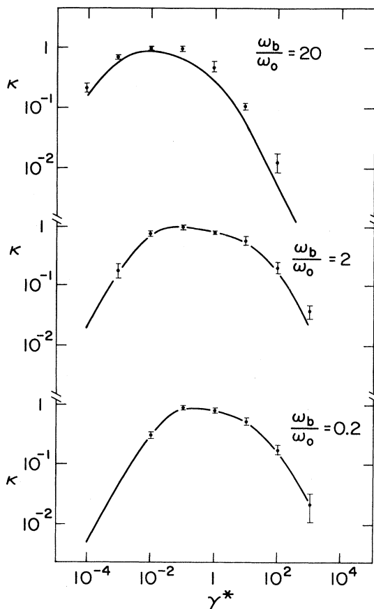
FIG. 19. Turnover in the presence of exponential memory friction [see Eq. (6.5)] as a function of the dimensionless damping \hat{\nu}(\omega=0)/\omega_b \equiv \gamma^* in the metastable potential of Eq. (6.6) for various frequency ratios, with \omega_b denoting the barrier frequency and \omega_0 the well frequency, respectively: solid circles with error bars, the SBB transmission coefficient data (Straub, Borkovec, and Berne, 1986) for a single-well potential; solid lines, the theory of Pollak, Grabert, and Hänggi (1989). The data are for an Arrhenius factor of \beta E_b = 20 , and \alpha^* = \alpha\omega_b^2 = \frac{4}{3} .
