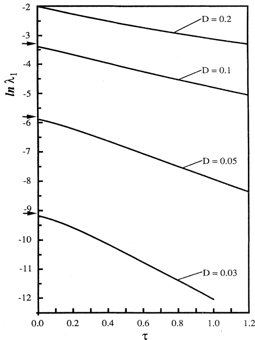
FIG. 35. Plot of the lowest eigenvalue \lambda_1(\tau)=2k(\tau) at small-to-moderate noise color \tau \leq 1.2 for various noise strengths D . The arrow indicates the steepest-descent approximation of the Smoluchowski rate k_S at zero noise color. After Jung and Hänggi (1988).
