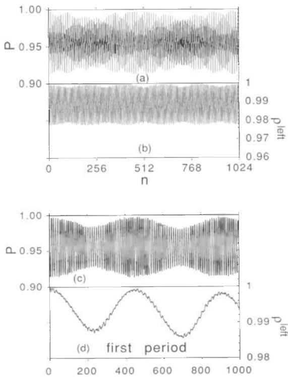
Fig. 1. Driven tunneling at an exact crossing of the two “lowest” quasi-energies (see text): (a) time evolution (quantum map), over the first 10^3 time steps, T = 2\pi/\omega , of the autocorrelation function P_n and (b) the occupation probability \rho_n^{\text{left}} in the initially populated well; resolution of the first period of P_n (c) and \rho_n^{\text{left}} (d) into 1000 time steps. The parameter values are \omega = 0.01 and S = 3.17 \times 10^{-5} .
