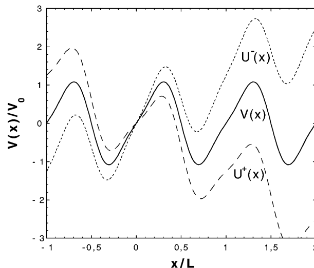
FIG. 1. Solid line: ratchet potential V(x) in (2). Dashed and dotted lines: tilted washboard potentials U^\pm(x) in (4) with Fl = 0.2V_0 , l = L/2\pi . Note that the extrema and the separating barriers are different for U^+(x) and U^-(x) , while the period L is in common.
