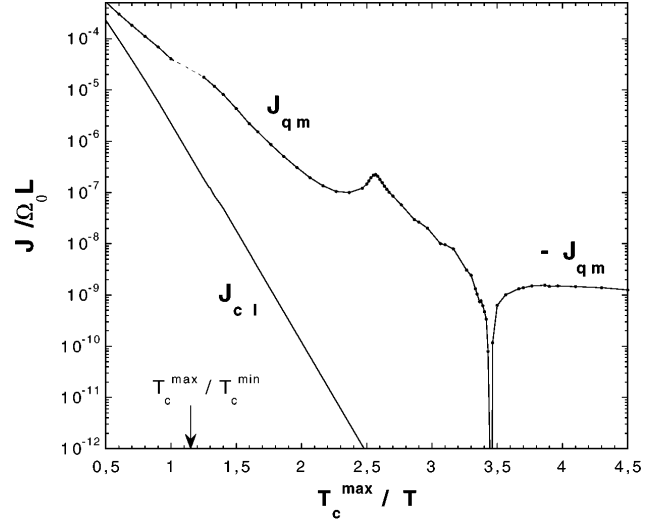
FIG. 2. The classical steady state current J_{cl} and its quantum mechanical counterpart J_{qm} for the ratchet potential from Fig. 1 in dimensionless units J/\Omega_0 L . Note the change of sign, the finite T = 0 limit, and the nonmonotonicity of J_{qm} . For more details, see main text.
