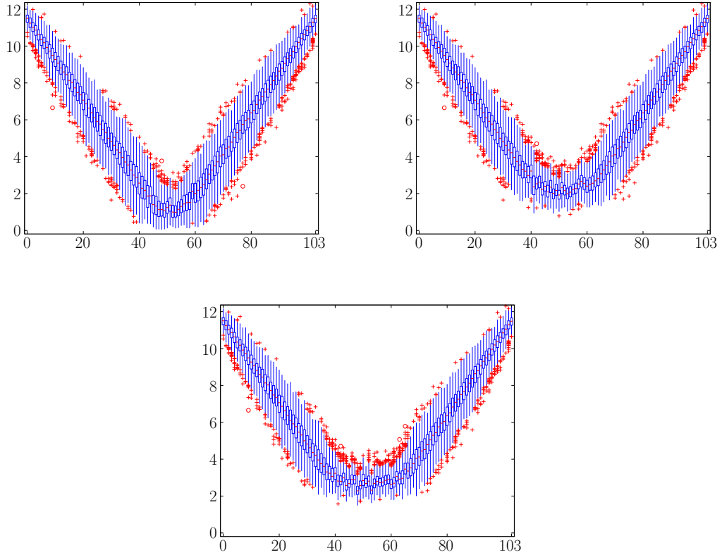
Figure 4: Boxplot of Monte Carlo simulations to determine typical values of the restricted norm ratios \|g^{(m)}\|_{L^\infty(0,c)} / \|g^{(m)}\|_{L^2(0,1)} for varying values of c . In all images, the horizontal axis represents the sign forcing parameter m , and for each m we performed N = 150 simulations. All graphs are for \varepsilon = 10^{-3} , and from top left to bottom middle we consider the cases c = 0.01 , c = 0.1 , and c = 0.3 , respectively.
