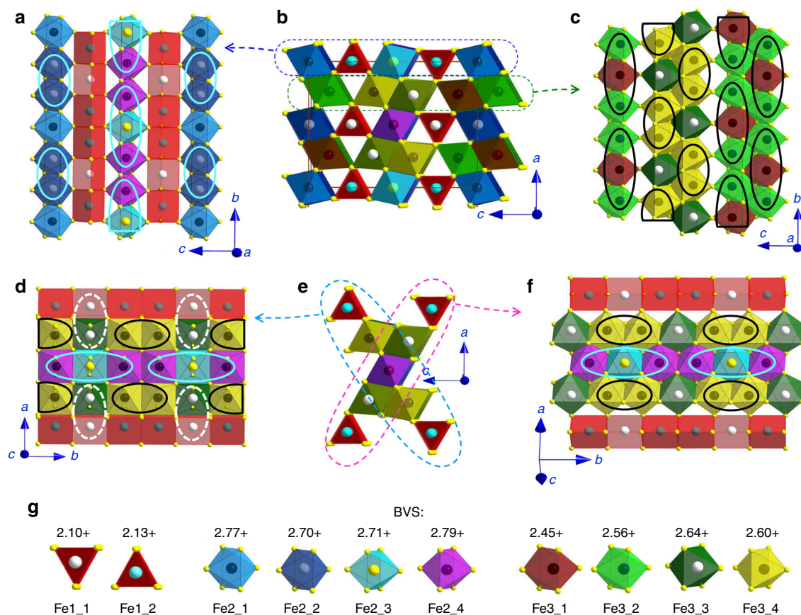
Fig. 4 Monoclinic crystal structure of \text{Fe}_4\text{O}_5\text{-III-a} . This structure has C2/m symmetry and plots are based on the crystal structure data refined at 11.7 GPa and 180 K. a Projection of the trigonal prisms Fe1 and single chains of Fe2 octahedra. b The unit cell projected down the b -axis. Thin solid lines indicate the unit cell edges. c Projection of the double chains of Fe3 octahedra. d Projection down the c -axis of one of the two diagonal ribbons shown in e . e Two characteristic diagonal ribbons consisting of five iron chains each. f Projection of one of two diagonal ribbons shown in e . Solid ellipsoids are dimers and trimers formed in the chains of octahedrally-coordinated iron. Dotted ellipsoids highlight Fe3-Fe1 pairs with shortened Fe-Fe length. Different crystallographic positions are shown in different colors. g Bond valence sums (BVS) values of all the iron cations in the crystal structure
