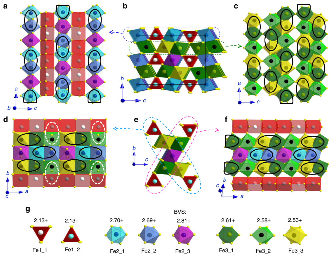
Fig. 5 Orthorhombic crystal structure of \text{Fe}_4\text{O}_5\text{-III-b} . The structure has \text{C22}_1 symmetry and plots are based on the crystal structure data refined at 11.7 GPa and 180 K. a Projection of the trigonal prisms Fe1 and single-chains of Fe2 octahedra. b The unit cell projected down the a -axis. Thin solid lines indicate the unit cell edges. c Projection of the double chains of Fe3 octahedra. d Projection down the c -axis of one of the two diagonal ribbons shown in e . e Two characteristic diagonal ribbons consisting of five iron chains each. f Projection of one of the two diagonal ribbons shown in e . Solid ellipsoids are dimers formed in the chains of octahedrally-coordinated iron. Dotted ellipsoids highlight Fe3-Fe1 pairs with shortened Fe-Fe length. Different crystallographic positions are shown in different colors. g Bond valence sums (BVS) values of all the iron cations in the crystal structure
