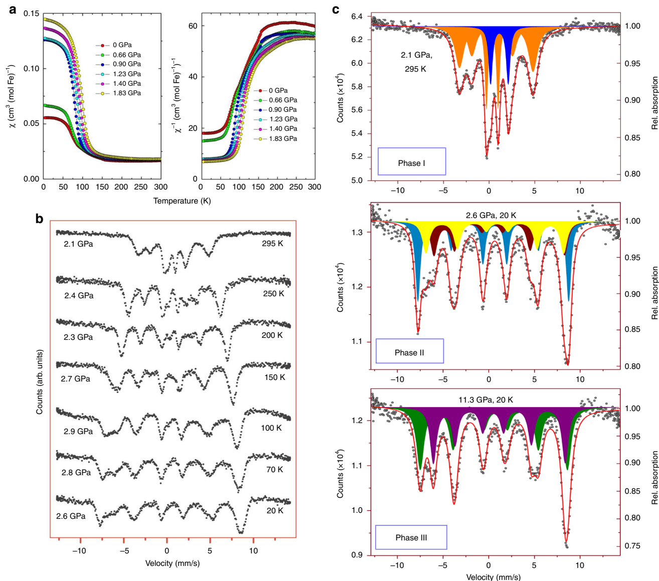
Fig. 8 Magnetic susceptibility and Mössbauer spectra of \text{Fe}_4\text{O}_5 . a Temperature dependence of magnetic susceptibility and inverse magnetic susceptibility measured at different hydrostatic pressures in a field of 0.5 T under field cooling. b Evolution of Mössbauer spectra upon cooling at about 2–3 GPa. Broadening of the first (low-velocity) line of the sextet starting at 150 K indicates charge ordering. c Representative Mössbauer spectra of different phases of \text{Fe}_4\text{O}_5 collected at different pressures and temperatures. The spectrum of phase I can be refined by superposition of a paramagnetic doublet (blue) assigned to iron in the trigonal prisms and a magnetic sextet (orange) assigned to Fe in the octahedra in a mixed-valence state. The spectra of phases II and III exhibit a complex distribution of hyperfine fields and can be refined by superposition of sextets
