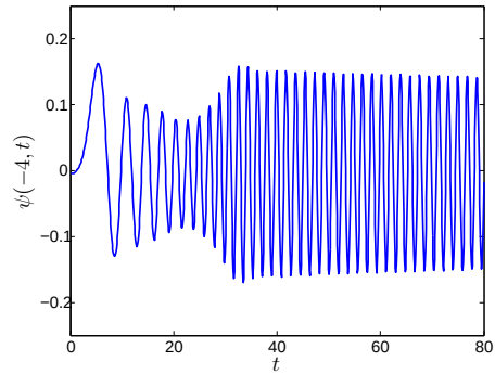
Fig. 1: Time evolution of the free surface displacement at x = -4 for plate with fixed top.
