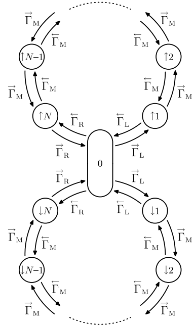
Fig. 5. The situation depicted in Fig. 4 is generalized to include the electron spin. The two rings corresponding to the two spin directions are joined via the neutral state “0” of the molecule.
