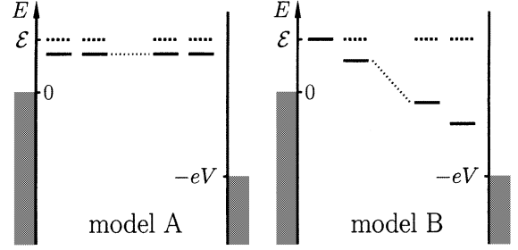
Fig. 3. The positions of the energy levels are shown for models A (left) and B (right) of the voltage drop across the system.
