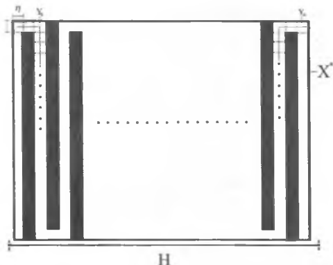
FIG. 2. Filamented domain partitioned with squares and showing the longest paths.
