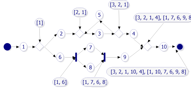
Fig. 4. The calculated sets of minimally executed actions for this workflow.
