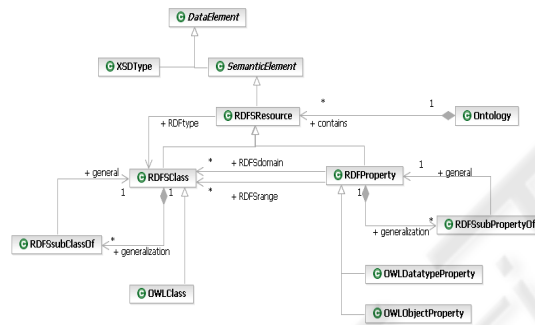
Figure 4: SWS meta-model for the ontology.
