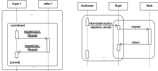
Figure 4. nested protocol and interleaved protocol
