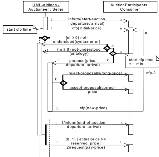
Figure 1. English-Auction protocol for surplus flight tickets
