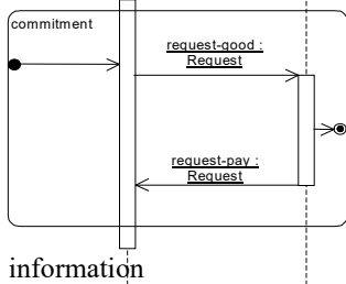
Figure 5. Input/output of nested protocols
