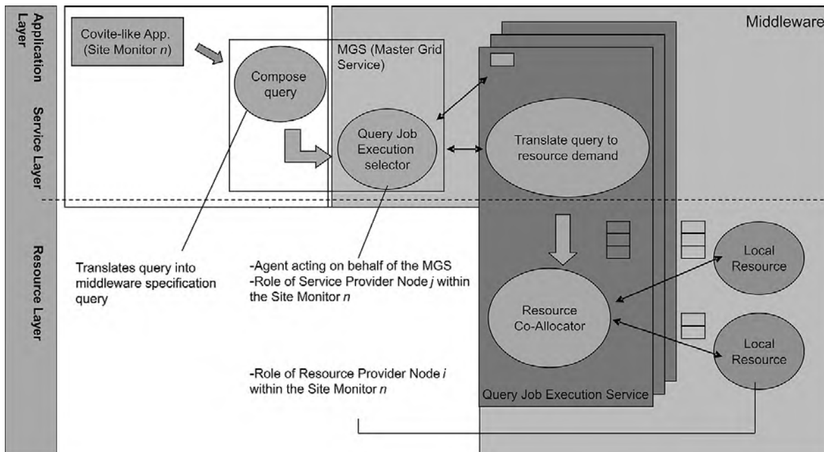
Fig. 5. The proposed multiagent system architecture for indexing and querying.
