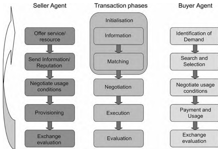
Fig. 2. Lifecycle of agents.
