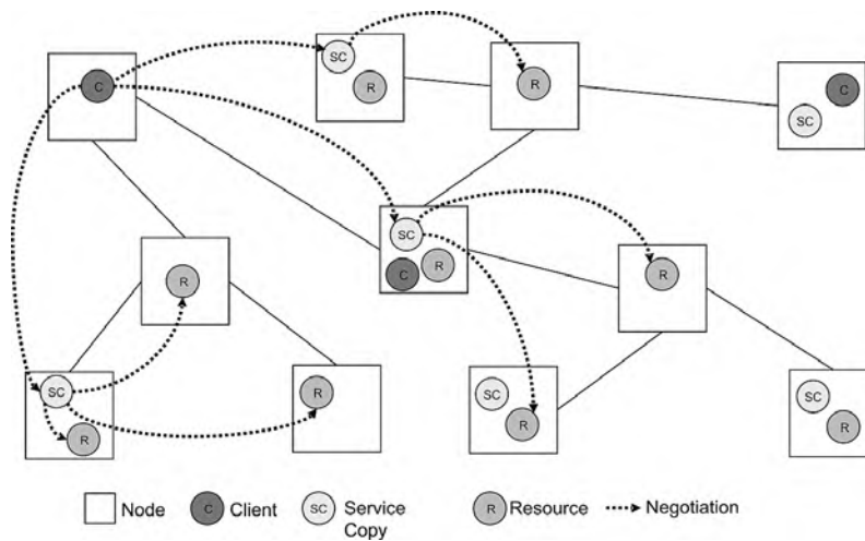
Fig. 3. Catalallactic middleware as a network of agents.
