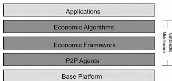
Fig. 4. Layered agent architecture.
