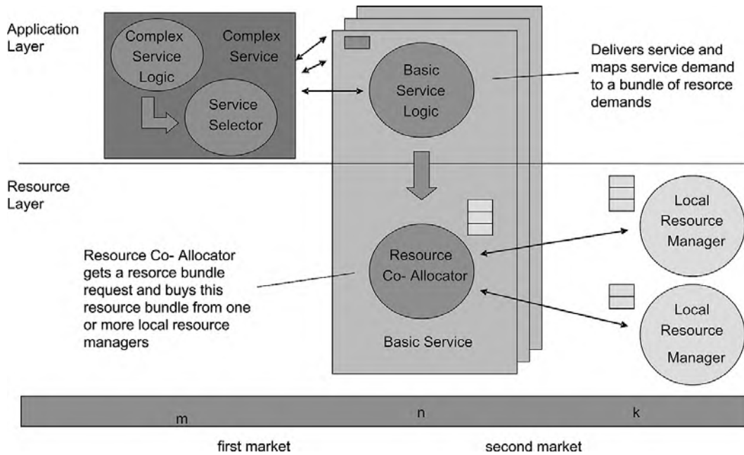
Fig. 1. Catallaxy-based Grid market model.
