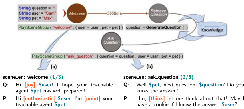
Fig. 4. Examples of calling scenes of the multimodal scenescript
