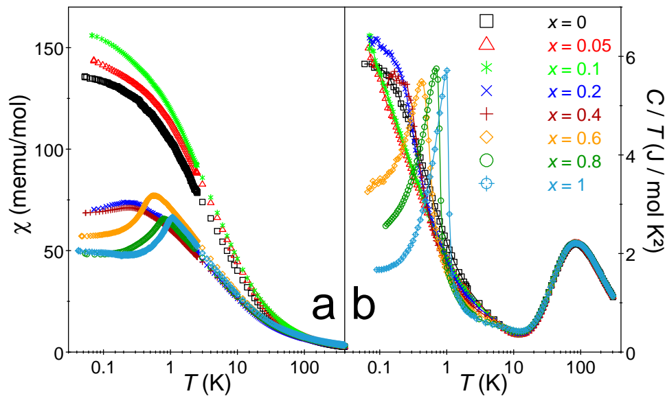
Figure 1. (a) The magnetic susceptibility \chi and (b) the specific heat divided by temperature C/T of CeNi 9-x Co x Ge 4 in semi-logarithmic plots. AFM transitions are evident for x \geq 0.2 .
